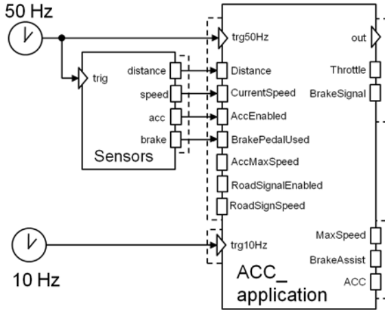
Fig. 8. The ACC specification obtained from the execution of Ao2ProCom
