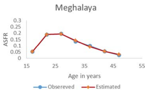
Figure 2. The Plot of Observed and Estimated ASFR of Meghalaya.
