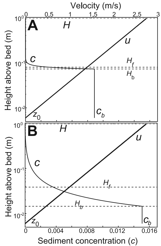
Figure 1. Schematic showing vertical profiles of sediment concentration c (equation (26)) and velocity u (equation (21)) for the conditions of the Eel River (Table 1) and for (a) 60-mm gravel and (b) 1-mm sand. Also shown are the calculated heights of the bed load layer H_b (equation (25)), weighted average particle fall heights H_f (equation (32)), flow depth H (Table 1), and the near-bed sediment concentration c_b (equation (18)).
