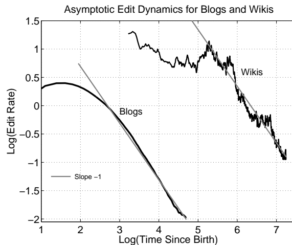
Fig. 2. The asymptotic decay in edit rate. The thin straight lines with slope -1 correspond to 1/t decay. The optimal linear fits to the tail of the blog data and Wikipedia data had slopes of -1.03 and -0.98 respectively. The tail for the blogs was the edit dynamics from about 1 hour to about 9 hours after birth, and for the wikis it was the edit dynamics from 450 days to 1400 days from birth.
