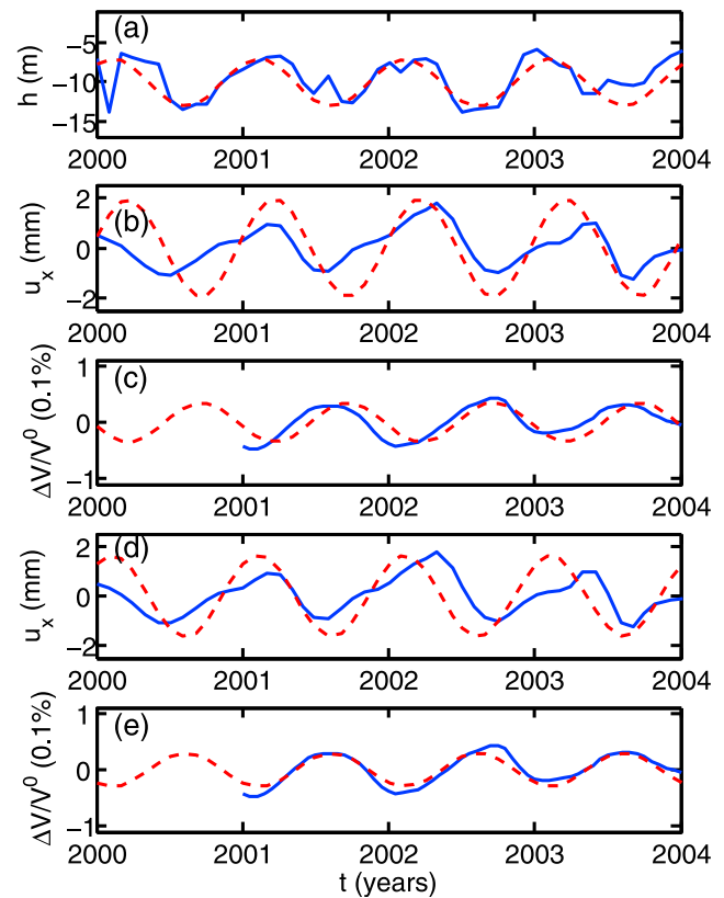
Figure 4. Comparison of observed (solid blue) and modeled (dashed red) quantities from water table variability. (a) Water table record from California state well 04S12W36J001S in Rossmoor, California ( http://www.water.ca.gov ) and modeled water table with h_0 = 3 m, corresponding to p_0 = 2.9 \cdot 10^4 Pa. (b and c) Comparisons equivalent to those in Figures 3b and 3c but for poroelastic effects. (d and e) Comparisons equivalent to those in Figures 3b and 3c but for direct elastic effects. Both Figures 4c and 4e use the less extreme choice of m/\mu = 2 \cdot 10^3 .
