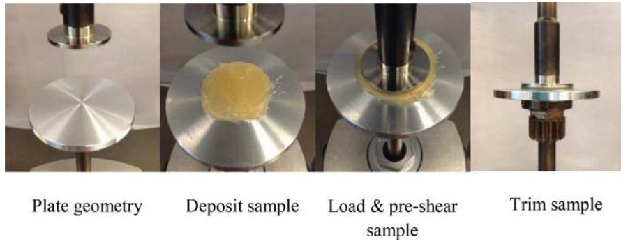
Figure 2. Loading and preshear procedure.
