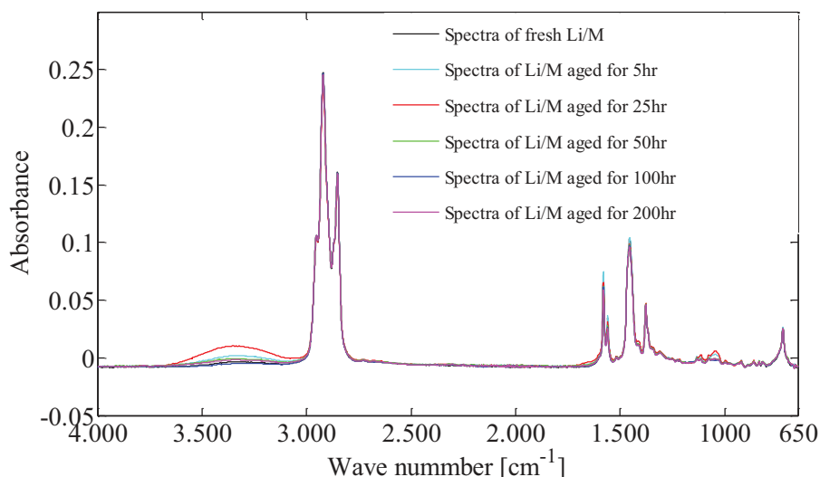
Figure 5. FTIR spectra of fresh and aged Li/M.
