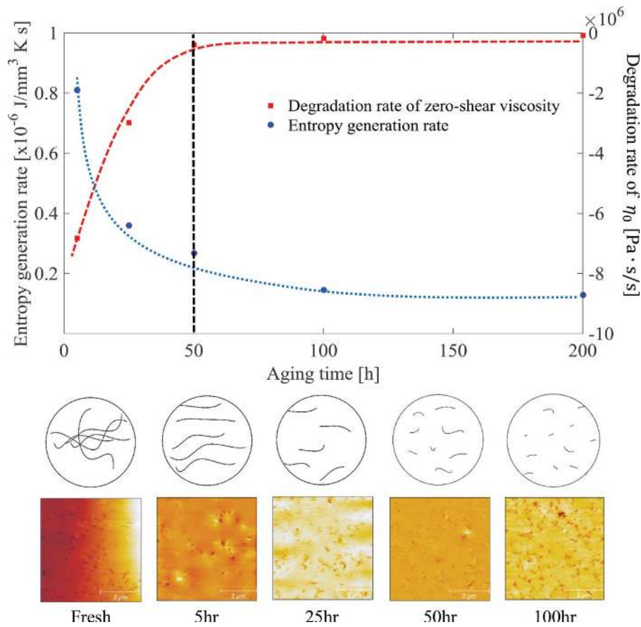
Figure 9. Aging of Li/M; cartoon and AFM results for different aging stages.
