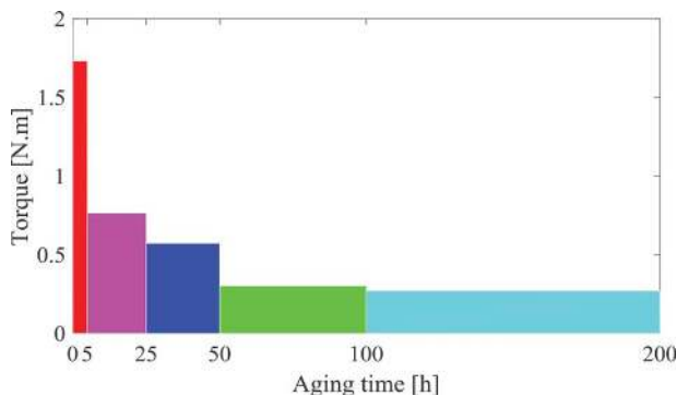
Figure 4. Calculated torque distribution for LiM aged at 83 rpm for 200 h.
