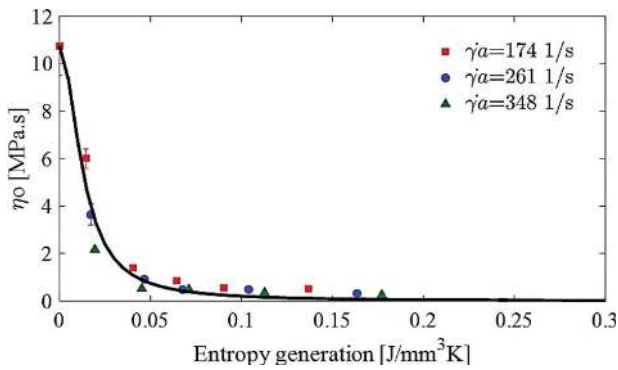
Figure 7. Zero-shear viscosity variation versus entropy generation density for Li/M.
