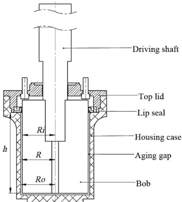
Figure 1. Couette aging test rig.
