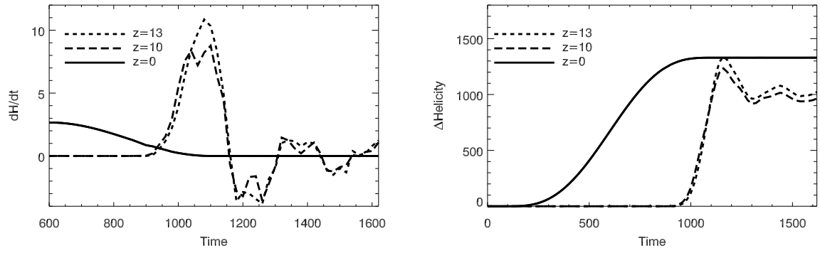
Fig. 11.— Fluxes ( left ) and time-integrated variations ( right ) of the magnetic helicity through horizontal xy planes at z = 0, 10 , and 13 .
