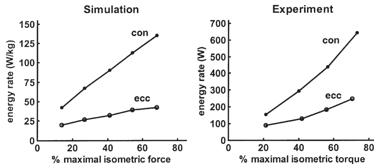
FIGURE 4 Dependence of total energy rate on intensity level during simulated and experimental concentric and eccentric cyclic contraction performed at the same rate. Simulation data are shown for the vasti group, while experimental data are from Hawkins and Molé [16], and were estimated from pulmonary oxygen consumption. The cycle rate for vasti was consistent with the cyclic knee extension/flexion rate used for the experimental data ( 90^{\circ}\text{s}^{-1} ). In both cases, total energy rate was approximately four times more sensitive to force production for concentric contractions than for eccentric contractions.
