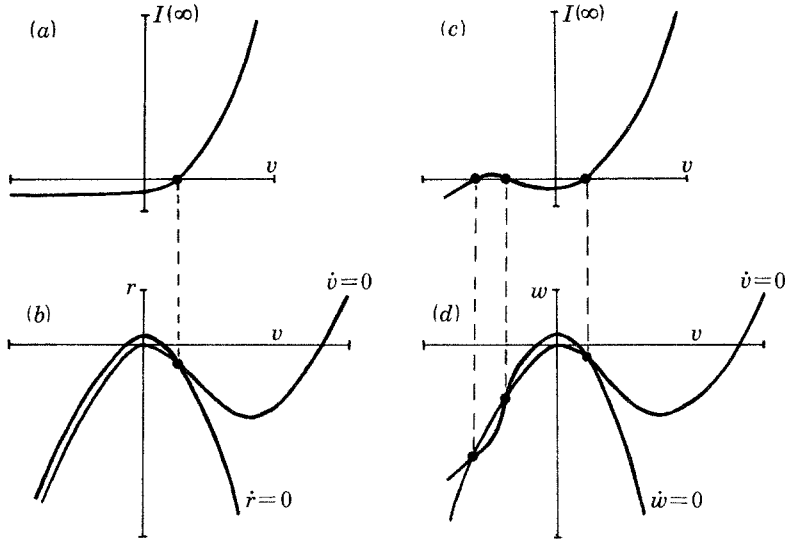
FIGURE 1. Schematic illustration of steady state current-voltage ( I(\infty) - v ) curves ( a ) for the one equilibrium point model, and ( c ) for the three equilibrium point model, and the corresponding v and r nullclines in the phase plane, ( b ), and v and w nullclines in the phase plane, ( d ).
