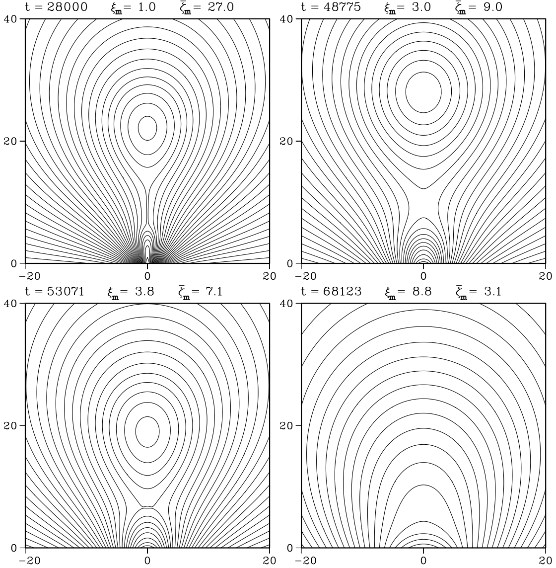
Fig. 11.— Destruction of the magnetic island in a magnetic arcade undergoing a shear-reducing, diverging footpoint motion (Case 4). In this case, we first impose a shearing footpoint motion for \eta = 10^{-5} to create a magnetic island. Then, we turn off the shearing motion and impose a diverging footpoint motion with V_{x0} = 10^{-3}v_0 at x = \pm 18 to reduce the relative plasma displacement. The magnetic island disappears at \bar{\zeta}_m \sim 6 .
