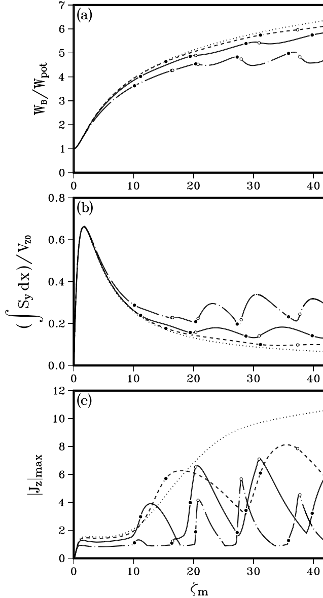
Fig. 5.— The evolution of (a) magnetic energy in units of the potential field energy, (b) Poynting flux through the bottom boundary divided by V_{z0} , and (c) maximum magnitude of the current density in the current sheet under the magnetic island for Case 1’s. All the quantities are plotted as a function of \zeta_m which is the plasma displacement at x = \pm 1 . In all three figures, the solid lines represent Case 1A in which V_{z0} = 10^{-3}v_0 and \eta = 10^{-5} , the chain-dotted lines represent Case 1B in which V_{z0} = 10^{-3}v_0 and \eta = 5 \times 10^{-5} , and the dashed lines represent for Case 1C in which V_{z0} = 5 \times 10^{-3}v_0 and \eta = 10^{-5} . The dotted lines are for the ideal MHD case (Case 1D) in which V_{z0} = 10^{-3}v_0 and \eta = 0 . The filled circles denote the initiation of a new reconnection event in the underlying arcade and the blank circles indicate the completion of the island merging.
