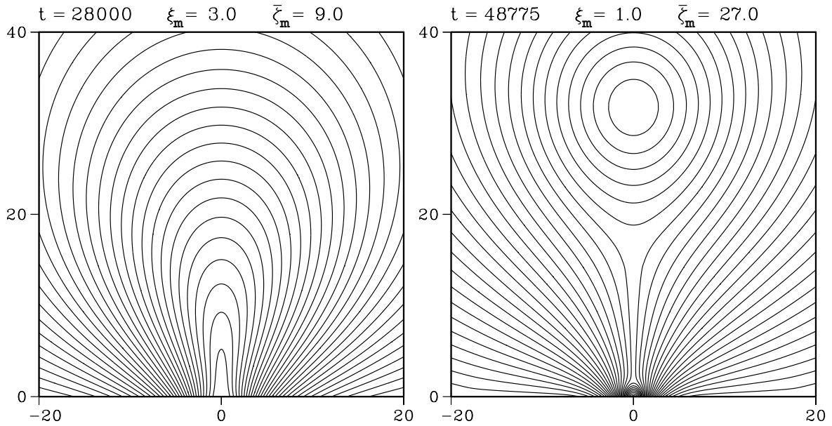
Fig. 7.— The resistive evolution of a magnetic arcade under a converging footpoint motion for \eta = 10^{-5} (Case 2A). In this case, a shearing footpoint motion parallel to the polarity inversion line with V_{z0} = 10^{-3}v_0 is first imposed for \bar{\zeta}_m = \zeta_m/\xi_m < 9 . Then, a purely converging footpoint motion given by equation (46) is applied to the arcade to further increase the relative plasma displacement.
