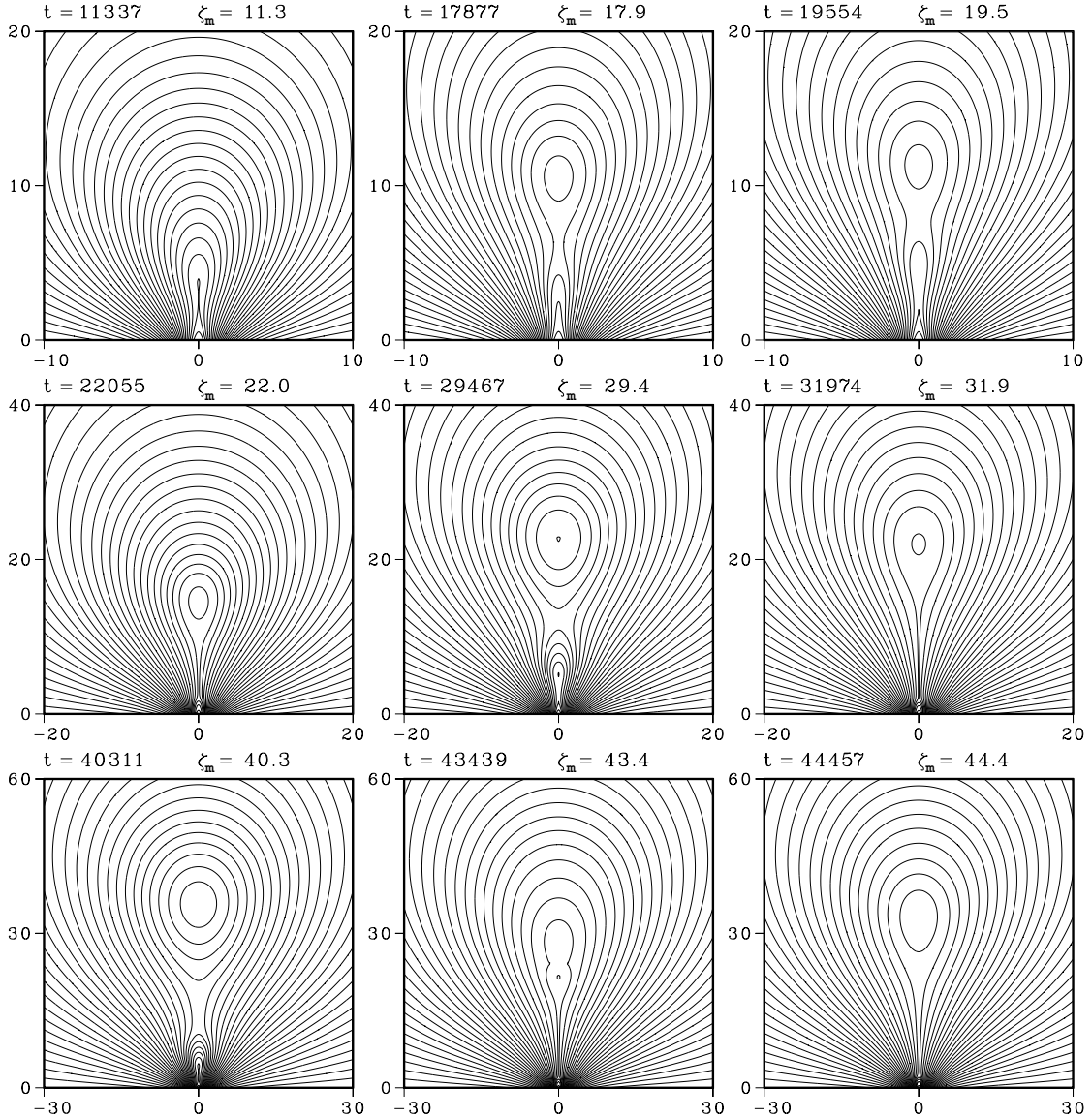
Fig. 3.— Repeated formation of magnetic islands and their merging under continuous footpoint shearing for Case 1A. Field lines projected on the xy -plane are shown for different times. Note that the figure scale increases row by row. The plasma displacement in the z -direction at the boundary normal field maxima ( x = \pm 1 ) is denoted by \zeta_m .
