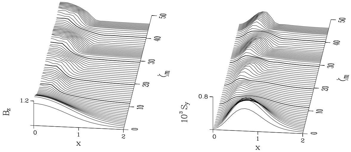
Fig. 6.— The toroidal magnetic field ( B_z ) and the upward component of the Poynting vector ( S_y ) in Case 1A plotted along the bottom boundary ( 0 \leq x \leq 2, y = 0 ) for different plasma displacements ( \zeta_m ), which is almost proportional to time. Thick lines indicate the initiation of a new reconnection in the underlying arcade.
