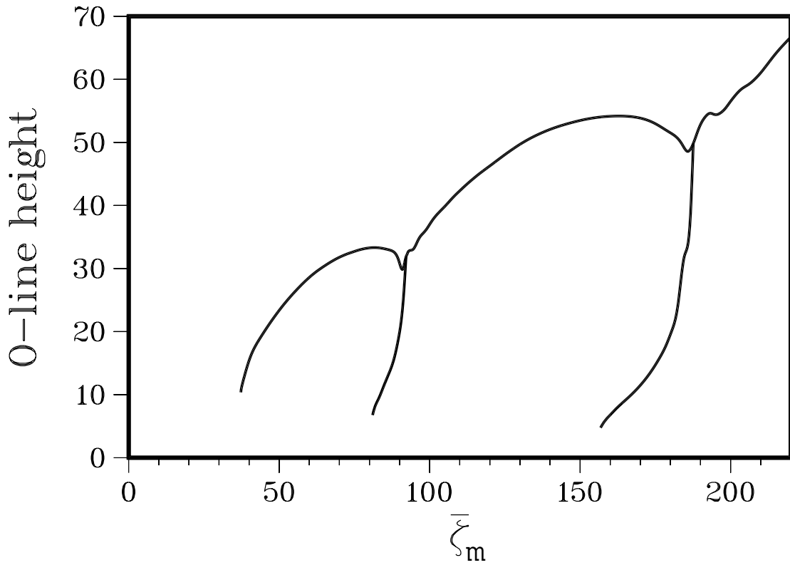
Fig. 10.— The height of O-lines in the magnetic islands in Case 3 as a function of \bar{\zeta}_m the relative plasma displacement at the boundary normal field maxima. Since \bar{\zeta}_m increases almost exponentially with time in this case, the rising speed of the magnetic islands increases more with shift in their generation than in Case 1.
