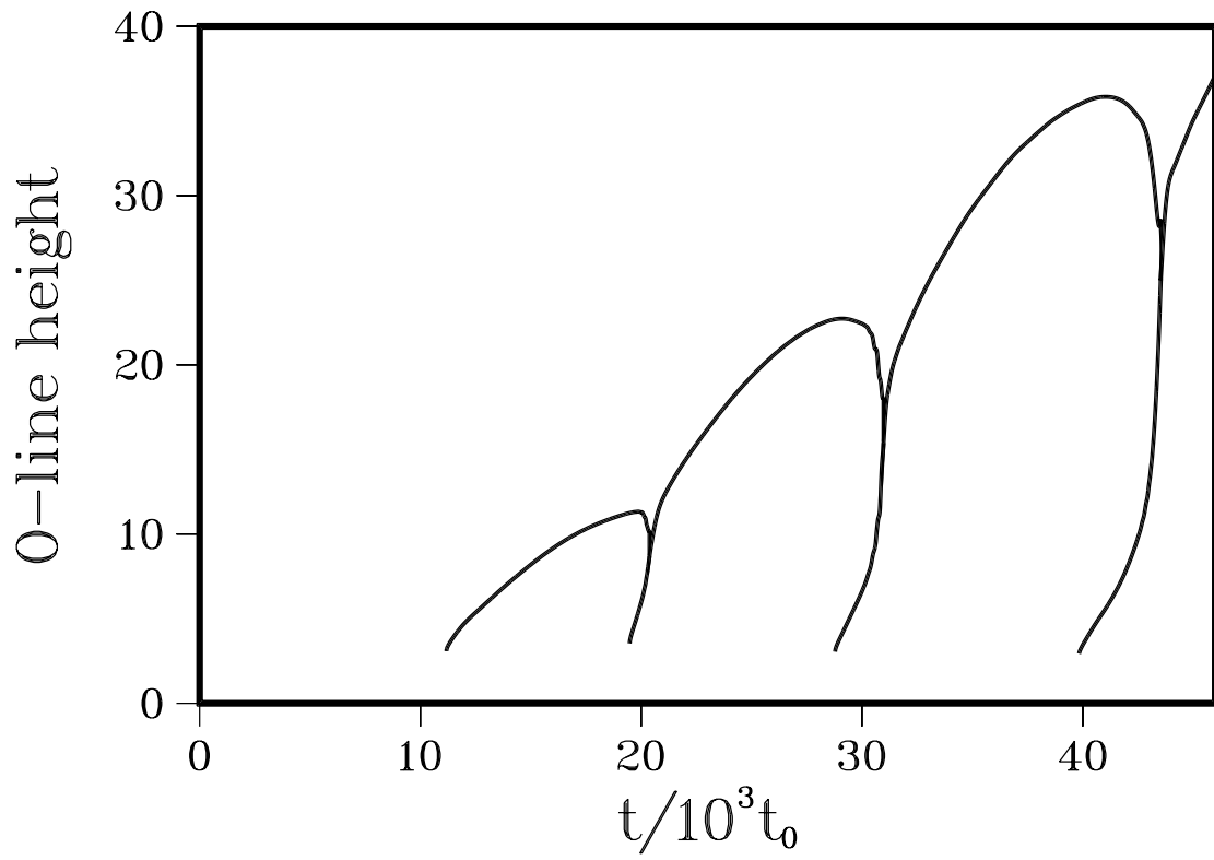
Fig. 4.— The height of O-lines of the magnetic islands in Case 1A as a function of time. The slope of the curves represents the rising speed of the magnetic islands.
