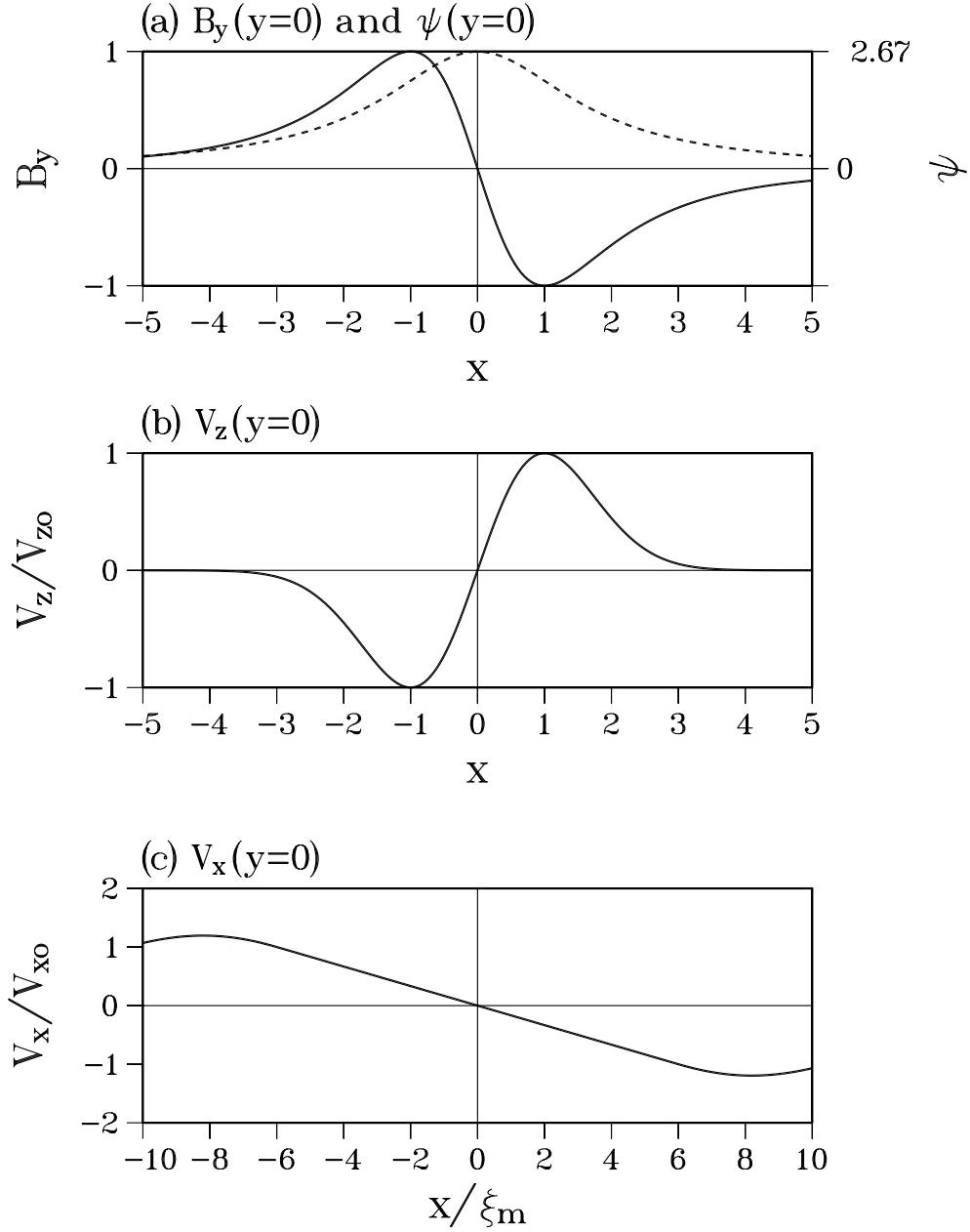
Fig. 2.— Profiles of (a) boundary normal magnetic field (solid line) and flux through the bottom boundary (dashed line), (b) shearing velocity in the z -direction, and (c) converging (or diverging) velocity in the x -direction. The normalization of all the quantities is given in table 1.
