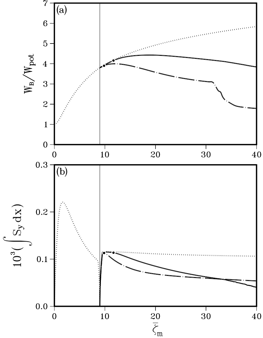
Fig. 8.— (a) The magnetic energy in units of the potential field energy and (b) the Poynting flux through the bottom boundary as a function of \bar{\zeta}_m for Case 2's. In both figures, the solid lines represent Case 2A in which \eta = 10^{-5} and the chain-dotted lines represent Case 2B in which \eta = 5 \times 10^{-5} . The dotted lines represent the ideal MHD case (Case 2C). In all three cases, the same boundary velocity profile is imposed. The vertical line indicates the time at which the shearing motion ceases and the converging motion commences. The initiation of magnetic reconnection is marked with a filled circle.
