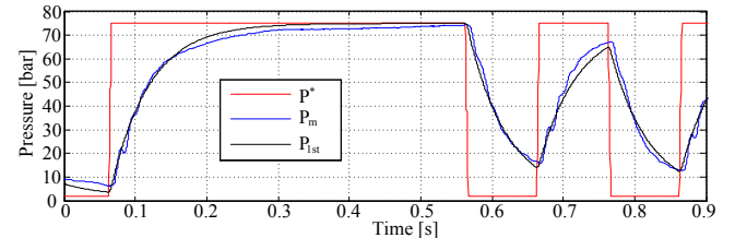
Figure 3: Comparison of the pressure responses of the control-oriented model from (7) denoted as P_{1st} with the real by-wire friction brake ( P_m : measured pressure). P^* is setpoint.
