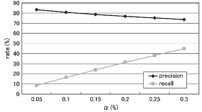
Fig. 4. Precision rate and recall rate of reliable frame selection.
