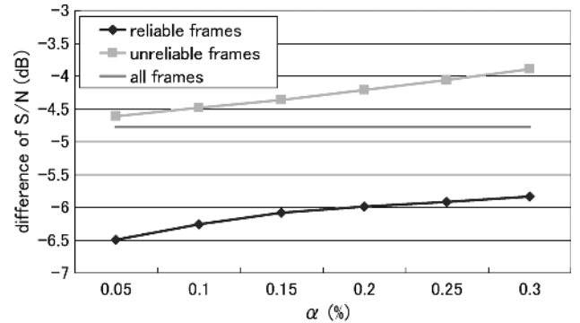
Fig. 5. Dependency of spectral distortion of selected frames on \alpha .
