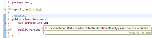
Figure 6: Primary key in a field not belonging to an entity.
