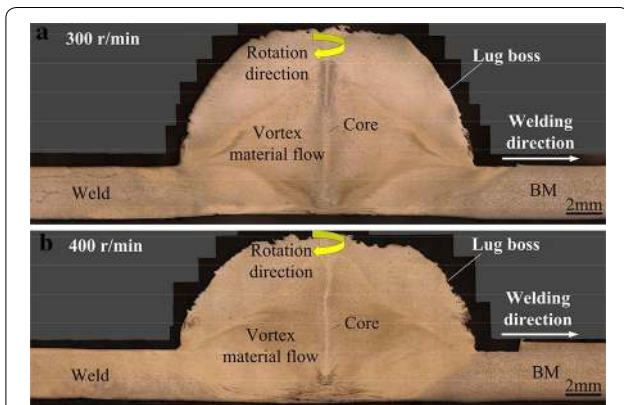
Figure 6 Macrostructure of the vortex material flow: a 300 r/min; b 400 r/min
