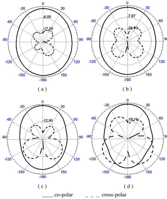
Figure 8. Measured radiation patterns ( H -plane, x - z plane ) of the proposed antenna at: (a) 4.2 GHz, (b) 5.2 GHz, (c) 5.8 GHz, and (d) 8.6 GHz.
