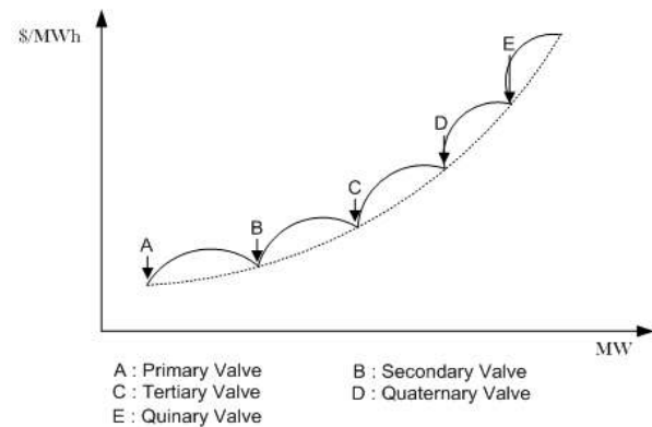
Fig. 1: Valve-point effect
