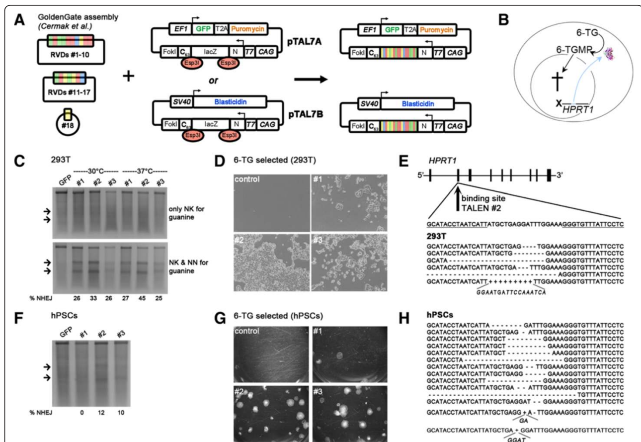
Figure 1 Pretesting of TALENs and mutational spectra in 293 T cells and hPSCs. A: Illustration of GoldenGate TALEN assembly by Cermak et al. [13] and cloning into new expression vectors pTAL7A and pTALB. Note that the number of RVDs is not limited to 18 but flexible. B: Schematic of negative selection of HPRT1 knock-out cells by 6-thioguanine (6-TG). 6-TG results in death of cells with functional HPRT1 . C: Cel-1 assay following transfection with three TALEN pairs (#1 to #3). Arrows indicate expected fragment sizes following Cel-1 digest of reannealed HPRT1 genomic PCRs (gPCR) as a result of error-prone NHEJ. Control plasmid (GFP) transfected cells served as negative control. Percentage of non-homologous end-joining (NHEJ) is indicated below each lane. D: Surviving 293 T cells following TALEN transfection and 6-TG selection of HPRT1 mutants. E: TALEN-induced mutation spectrum. Underlined wild-type sequence indicates binding region of TALEN pair #2. Mutant sequences shown are individual gPCR clones from bulk 6-TG selected cultures following transfection of TALEN pair #2. F: Pretesting of TALEN pairs #1 to #3 in HuES6 hESCs. Note that mutation efficiencies are somewhat decreased compared to 293 T cells in part B. G: Bulk hESC cultures following TALEN #2 transfection and 6-TG selection. H: TALEN-induced mutation spectrum in hESCs. All transfected cells were enriched by transient puromycin/blastocidin administration.
