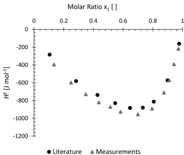
Fig. 8 Measured molar excess enthalpy H^E at 298.15 K for water (1) + methanol (2). With a slight offset, the obtained data nicely resembles measurements from literature. 10
