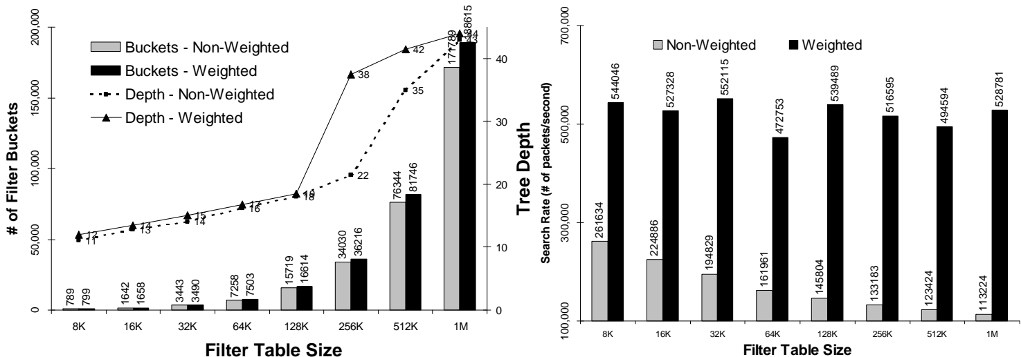
(a) Tree Statistics (b) Search Rate Fig. 8. Trends under various Filter Table Sizes (no jump table, filter bucket size = 16)
