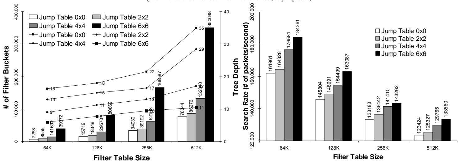
(a) Tree Statistics (b) Search Rate Fig. 10. Trends under various Filter Table Sizes with Jump Table (filter bucket size = 16)
