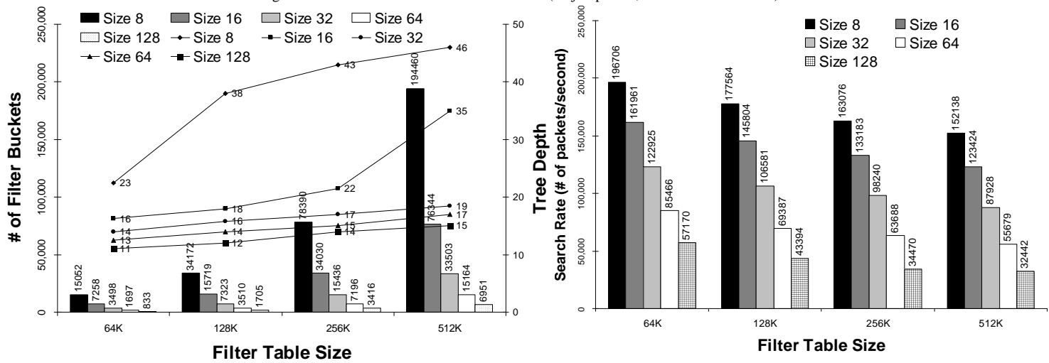
(a) Tree Statistics (b) Search Rate Fig. 9. Trends under various Filter Bucket Sizes (no jump table)
