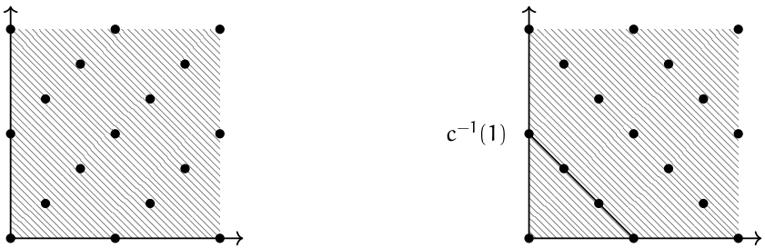
Figure 11. The monoid \mathbb{N}^2 \oplus_{\Delta, \mathbb{N}, d(e)} \mathbb{N} (on the left) and its dual cone for d(e) = 3 .
