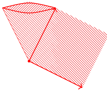
Figure 8. The cone space \text{Cone}(\Gamma) for \Gamma \in \mathcal{M}_{1,1}^{\text{trop}}(\mathbb{R}_{\geq 0}) a once-marked loop of edge length 1. A groupoid presentation of \text{Cone}(\Gamma) is shown in Figure 6 in red, as described in Example 4.10.
