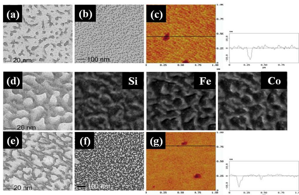
Fig. 18 (a, b)TEM images of a magnetic film following O 2 -RIE with (c) tapping-mode AFM image of a thin film on a Si substrate under similar conditions with sectional analysis (right). (d) TEM image of the same film with electron energy loss spectroscopy (EELS) elemental maps for Si, Fe, and Co. (e, f) TEM images of a magnetic film following H 2 -RIE with (g) tapping-mode AFM image of a thin film on Si under similar conditions with sectional analysis (right). Reprinted with permission from ref. 43. Copyright (2004) Wiley-VCH.
