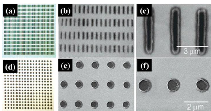
Fig. 10 (a) Optical micrographs and (b and c) scanning electron microscope (SEM) images of Mo-PFS microbars ( 0.5 \times 4.0 \mu\text{m}^2 ), (d) optical micrography and (e and f) SEM images of Ni-PFS microdots (diameter = 1.0 \mu\text{m} ). Images (e) and (f) were acquired with a 33^\circ stage tilt. Reprinted with permission from ref. 26. Copyright (2005) American Chemical Society.
