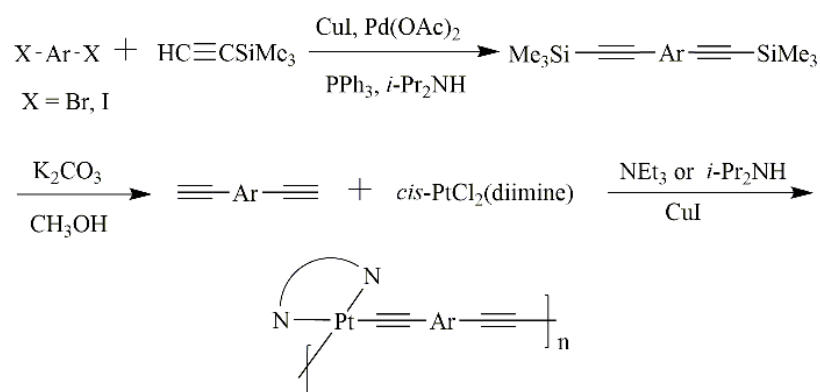
Scheme 1 General synthetic strategy of N, N' -coordinated polyplatinynes.
