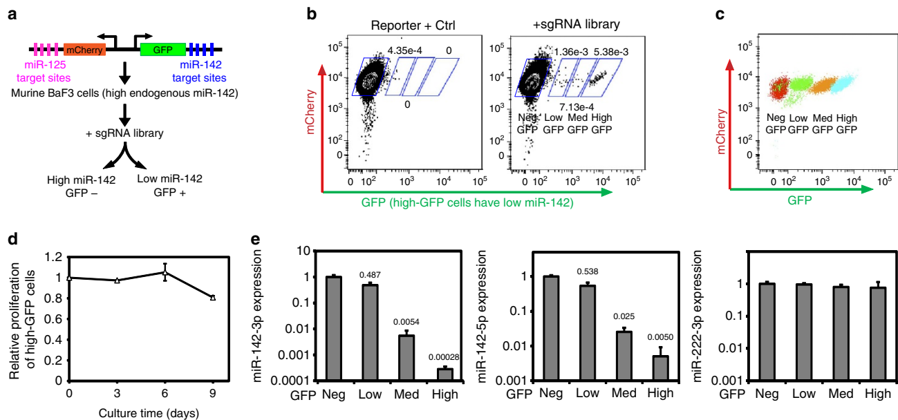
Figure 2 | A screen using the Molecular-Chipper-generated sgRNA library to identify both known and unknown functional cis-elements for miR-142 expression. (a) A diagram showing the miR-142 reporter design and the screen rationale. (b) Representative flow cytometry plots (out of three biological replicates) are shown for BaF3 miR-142-3p reporter cells transfected with a control vector or the sgRNA library. Number indicates the percentage of gated population. (c) Neg-, low-, med- and high-GFP cells were FACS sorted, and then resorted to improve purity. A representative flow cytometry plot is shown for the four indicated populations after sorting and resorting. (d) Competitive proliferation of high-GFP cells and neg-GFP cells was determined. Neg-GFP and high-GFP BaF3 miR-142-3p reporter cells (both mCherry positive) were FACS sorted and mixed with mCherry-negative BaF3 cells. The relative ratio of mCherry-positive to mCherry-negative cells was determined by flow cytometry at the indicated days. Data from high-GFP cells were normalized against those from low-GFP cells. N = 3 biological replicates. Error bars represent s.d. Note the absence of strong selection against high-GFP cells. (e) Mouse miR-142-3p, miR-142-5p and miR-222-3p expression levels in neg-, low-, med- and high-GFP populations (from samples in (c)) were determined by qRT-PCR. The relative expression levels are labelled relative to that in neg-GFP samples. Note that data are shown in log scale. Also note that the miR-222-3p expression is shown as a control. N = 3 technical replicates. Error bars represent s.d. Data are from a representative experiment out of two performed.
