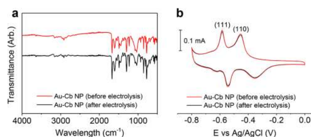
Figure 5. (a) FT-IR spectra of Au–Cb NP before and after electrolysis; (b) Pb-upd profiles of the Au–Cb NP before and after electrolysis. Scan rate: 50 mV/s.
