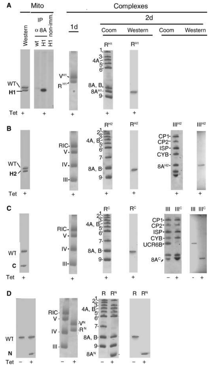
Figure 5. Effects of expressing RIC8A mutants on mitochondrial complexes of L. tropica . (A–D), Complexes in cells expressing H1, H2, C-terminal domain or N-terminal domain, respectively. Left to right: western blot of total mitochondrial protein resolved by Tricine-SDS-PAGE, and probed with polyclonal anti-RIC8A antibody; ^{35}\text{S} -methionine-labeled protein from wild-type or H1-expressing cells immunoprecipitated with nonimmune or anti-RIC8A serum; BN-PAGE profiles (Coomassie stain and western blot) of mitochondrial complexes; and subunit profiles (SDS-PAGE) of RIC and complex III. Subunit numbering as in ref. 9. Sizes of the endogenous (WT), H1 and H2 are 202, 195 and 185 amino acid residues, respectively.
