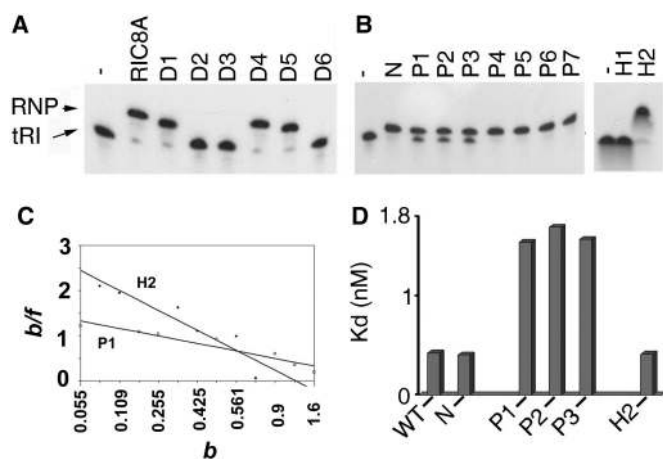
Figure 2. tRNA-binding activity of RIC8A mutants. (A and B) Gel-shift assays using 32 P-labeled tRNA Ile (tRI) (10 fmol) and wild-type (RIC8A) or indicated mutant recombinant proteins (100 fmol). RNP, ribonucleoprotein. (C) Examples of Scatchard plots for mutants H1 and P2. b , concentration of bound tRI; f , concentration of free RNA. (D) Dissociation constants ( K_d , nM) of complexes of tRI with indicated RIC8A derivatives. All variants are recombinant proteins expressed in E. coli . P1–P7 are derived from clone N (Figure 1) spanning residues 1–82.
