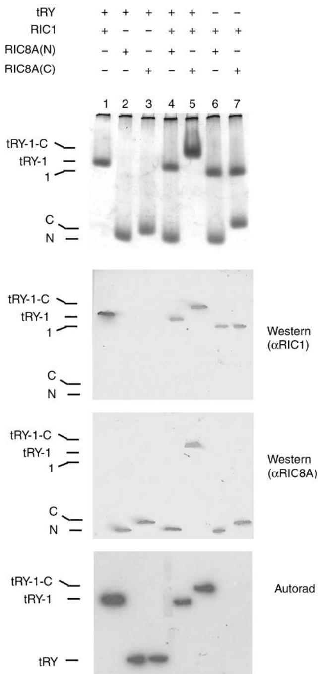
Figure 7. Interaction of the RIC8A C-terminal domain with RIC1. Recombinant proteins and ^{32}\text{P} -labeled tRNA Tyr were incubated in the indicated combinations and the products separated by native gel electrophoresis. (A) Coomassie stain. (B and C) parallel western blots probed with anti-RIC1 or anti-RIC8A antibody, respectively. (D) Autoradiogram.
