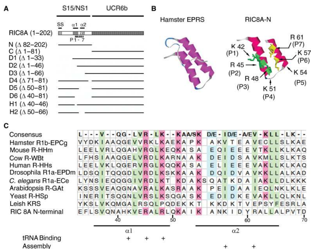
Figure 1. Domain structure and organization in RIC8A. (A) Domains and subdomains: ss, mitochondrial targeting sequence; \alpha 1 , \alpha 2 , the two helices of the S15/NS1-like domain. Positions of various deletions (D) and point mutations (P) are shown. (B) Homology model of RIC8A N-terminal domain (right) templated on the hamster GluProRS repeat R1. Side chains of residues altered to alanine are indicated (mutant numbers in parenthesis). (C) Sequence alignment of the \alpha 1 – \alpha 2 region of RIC8A with the appended S15/NS1 domain of eukaryotic aaRS. Different residue types are shaded differently: pink, basic; blue, acidic; green, hydrophobic. Residues involved in tRNA binding, or assembly, are indicated by + signs.
