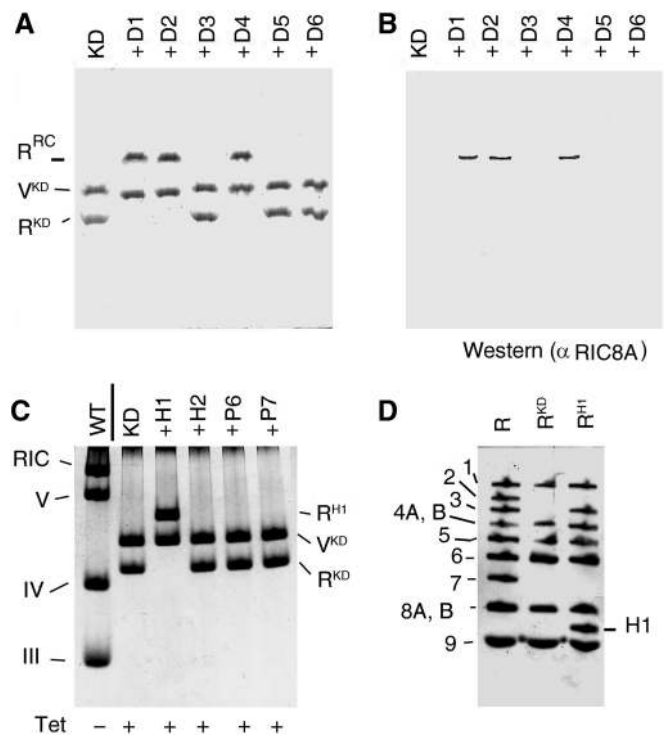
Figure 3. Assembly competence of RIC8A mutants in vitro . (A and C) BN PAGE of RIC8A-knockdown complex (KD) reconstituted with indicated mutant proteins. WT, complexes from uninduced cells, Coomassie stain. (B) Western blot of gel run in parallel to (A), probed with anti-RIC8A antiserum (1:50). The amount of protein loaded on this gel was about one-third that in (A). R KD , knockdown RIC subcomplex; V KD , complex V from KD cells; R RC , reconstituted RIC. (D) SDS-PAGE profile of R KD and R RC(H1) (RIC reconstituted with H1 protein), compared to wild-type RIC (R). RIC subunits are numbered as in ref. 9.
