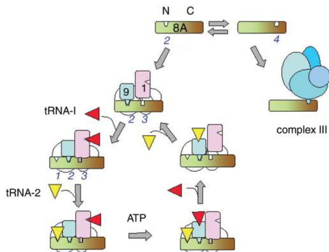
Figure 8. Schematic representation of the proposed role of the interaction motifs of RIC8A in assembly and import. Motifs 1–4 in RIC8A are lettered in blue. tRNA-I and tRNA-II are types I and II tRNAs, respectively. For details, see text.
