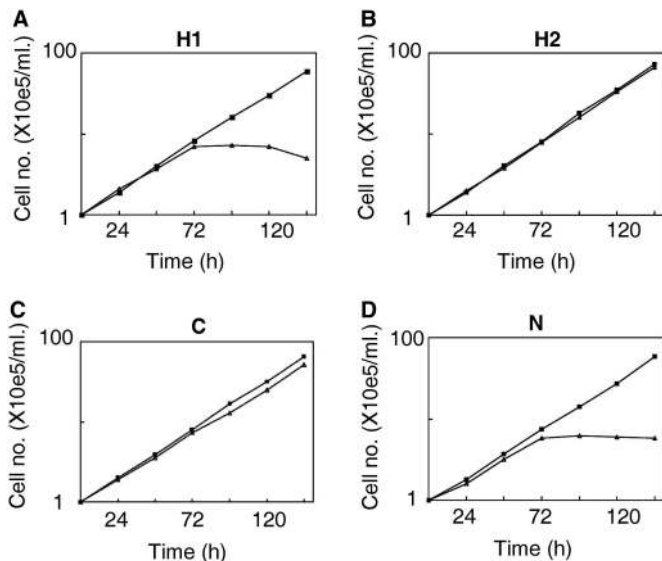
Figure 4. Growth curves of uninduced (squares) or tetracycline-induced (triangles) promastigotes transformed with RIC8A derivatives. (A–D) Deletion mutants H1, H2, C-terminal and N-terminal domain, respectively.
