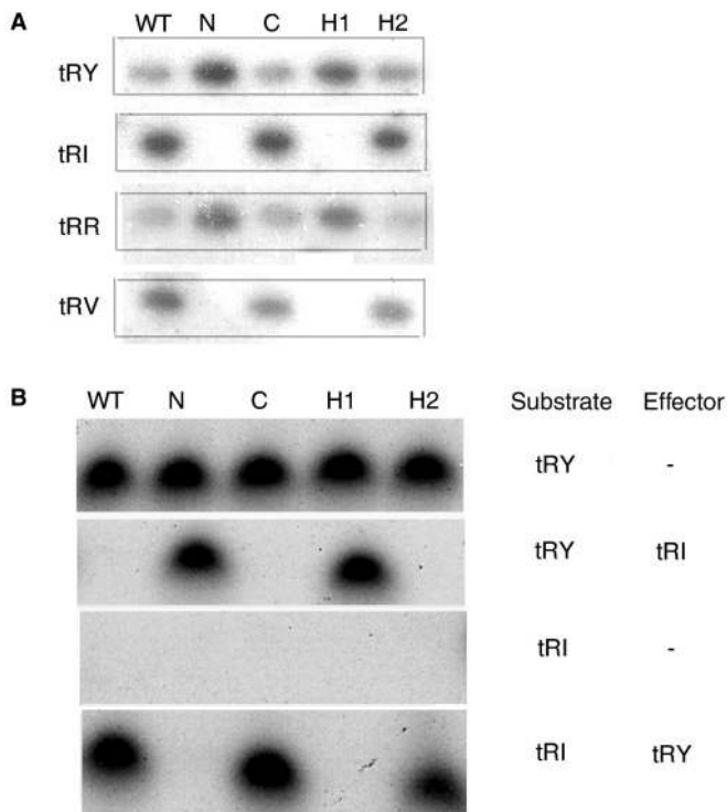
Figure 6. Effect of expressing RIC8A derivatives on tRNA import. (A) Nucleus-encoded mitochondrial tRNAs in normal (WT) or mutant RIC8A-expressing cells. Northern blot of mitochondrial RNA ( 5 \times 10^6 cell-equivalents) probed with antisense oligonucleotides complementary to the indicated tRNAs: tR(X), tRNA specific for amino acid X (single-letter code). (B) Import of indicated ^{32}\text{P} -labeled substrates, in the presence or absence of low-specific-activity effector, into liposomes reconstituted with extracts from RIC8A derivative-expressing cells (RNase protection assay).
