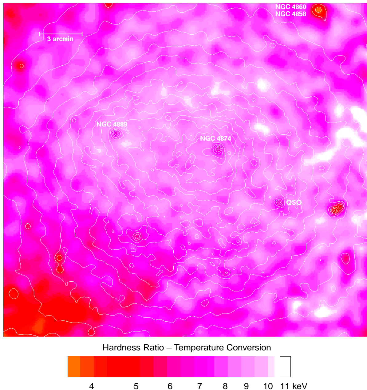
Fig. 3. The hardness ratio map of the inner Coma region in the energy bands from 0.3–2 keV and 2–7.15 keV. The overlain contours are from the smoothed surface brightness distribution in the energy band from 0.3–2 keV
