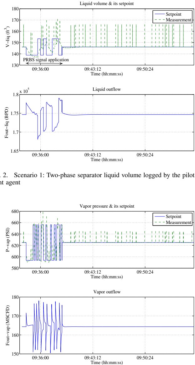
Fig. 3. Scenario 1: Two-phase separator pressure logged by the pilot plant agent
