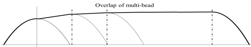
Fig.8 The schematic overlapped profile of a multi-bead deposit at d < d^*
