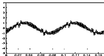
Fig.3b Triplen harmonic content, |V_{st}| = 0.2V_{dc}
