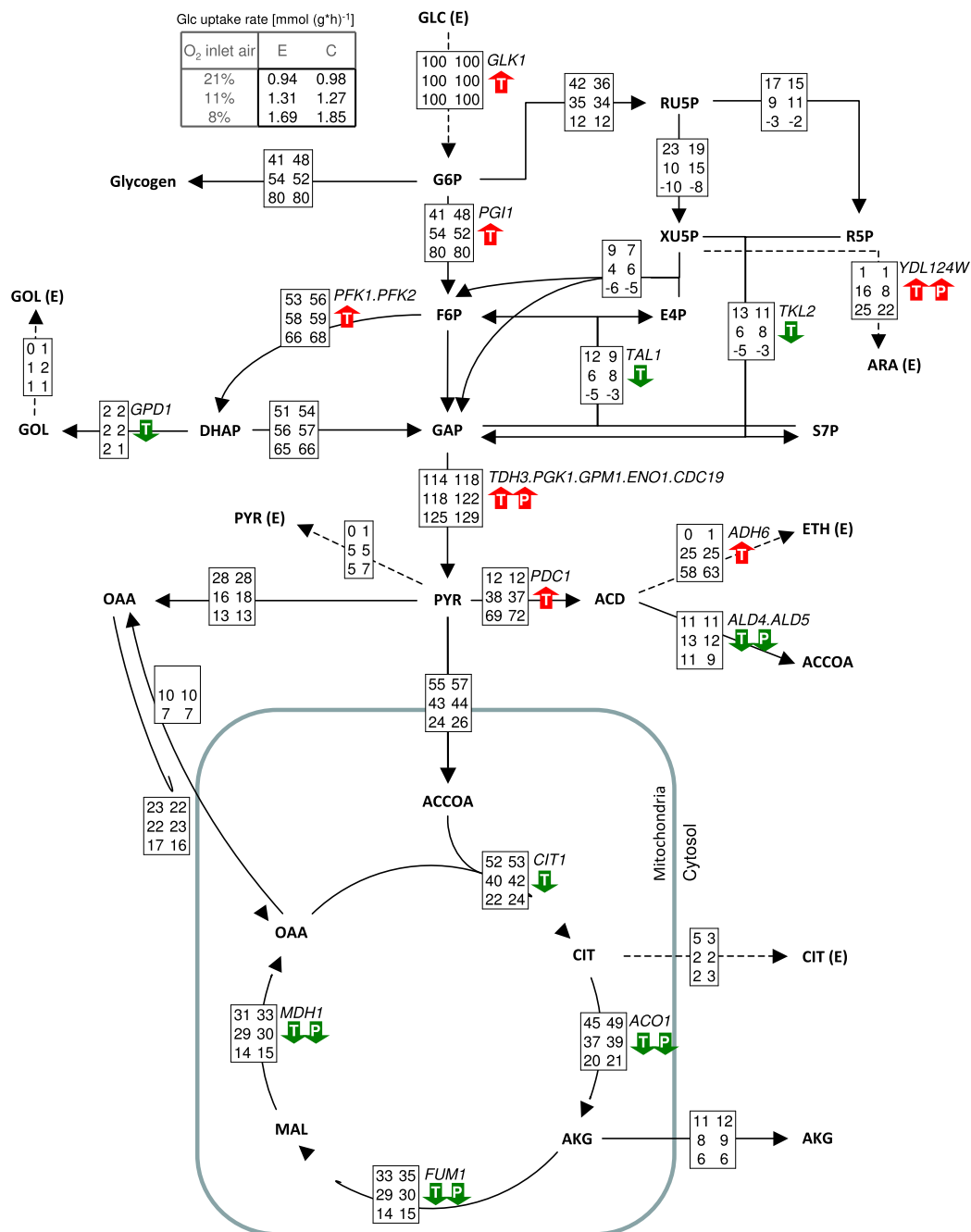
Figure 4 Metabolic flux distributions in P. pastoris Fab-expressing and control strains under different oxygenation conditions. Relative net flux distributions of P. pastoris X-33/pGAP \alpha _Fab and X-33/pGAP \alpha in glucose-limited chemostats at a D = 0.1 h -1 under different oxygenation conditions. Fluxes are shown as relative fluxes normalized to the specific glucose uptake rate (expressed as mmol glucose g -1 DCW h -1 ) in the corresponding experiment. The specific glucose uptake rates corresponding to the different oxygenation conditions and strains are given at the top of the figure. The fluxes for each reaction in the network corresponding to 21%, 11% and 8% oxygen in the bioreactor inlet gas are given from top to bottom; the flux values from the Fab-producing strain are shown on the left and those from the corresponding control strain on the right. The transport of Oaa across the mitochondrial membrane under normoxic conditions is given as a single net influx value. Fluxes with SD values are provided in the Additional file 5. Arrows indicate higher (red) or lower (green) mRNA levels (T) and protein abundances (P) during hypoxia compared to normoxia. The corresponding gene/protein names (in italics) are displayed above the arrows, while all metabolite names are indicated in bold letters: GLC = glucose; G6P = glucose-6-phosphate; F6P = fructose-6-phosphate; GAP = glyceraldehyde-3-phosphate; DHAP = dihydroxyacetone phosphate; GOL = glycerol; RU5P = ribulose-5-phosphate; XU5P = xylulose-5-phosphate; R5P = ribose-5-phosphate; ARA = arabinol; S7P = sedoheptulose-7-phosphate; PYR = pyruvate; ACD = acetaldehyde; ETH = ethanol; ACCOA = acetyl CoA; OAA = oxaloacetate; CIT = citrate; AKG = alpha-ketoglutarate; MAL = malate; (E) = external
