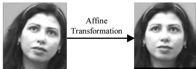
Figure 2. Normalization.
