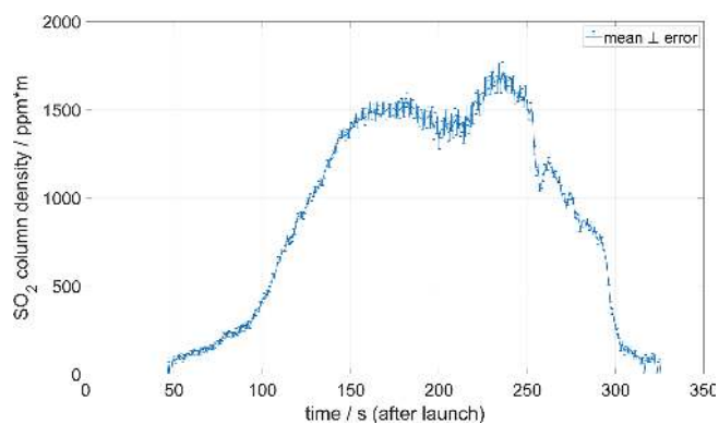
Figure 11. Example of MobileDOAS traverse made at Manam volcano on 27 May 2019 at an altitude of 1000 m a.s.l. The emission rate of \text{SO}_2 was 5200 \pm 660/180 \text{ t d}^{-1} , using the plume speed shown in Fig. 9. Information about the position of the drone below the plume is telemetered in real time.
