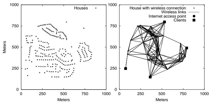
Fig. 19: (a) Houses in a suburban neighborhood (b) Formation of a mesh network in the suburban neighborhood among 35 randomly selected houses
