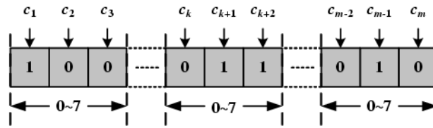
Figure 7. Bi-metrics Binary Representation - Composite encoding.
