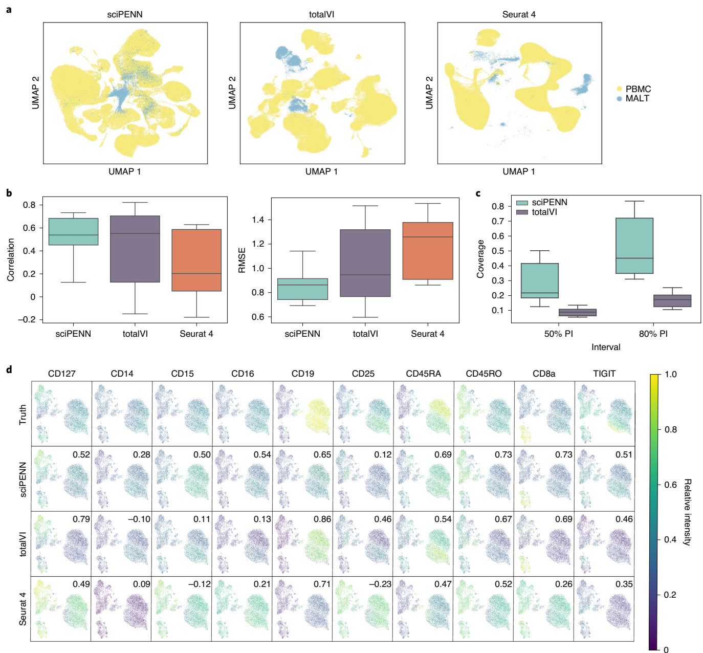
Fig. 2 | Protein expression prediction in the MALT dataset using the Seurat 4 PBMC dataset as reference. a , UMAP embeddings visualizing the integrated hidden representation of the data, for each method. Each cell is coloured according to the dataset from which it was sequenced. b , Box plots showing the correlation (left) and the RMSE (right) between each MALT protein's predicted and true values for each method. c , Box plots showing the empirical test coverage of nominal 50% and 80% PIs per protein computed with sciPENN and totalVI. In b and c , the lower and upper hinges correspond to the first and third quartiles, and the centre refers to the median value. The upper (lower) whiskers extend from the hinge to the largest (smallest) value no further (at most) than 1.5 \times interquartile
