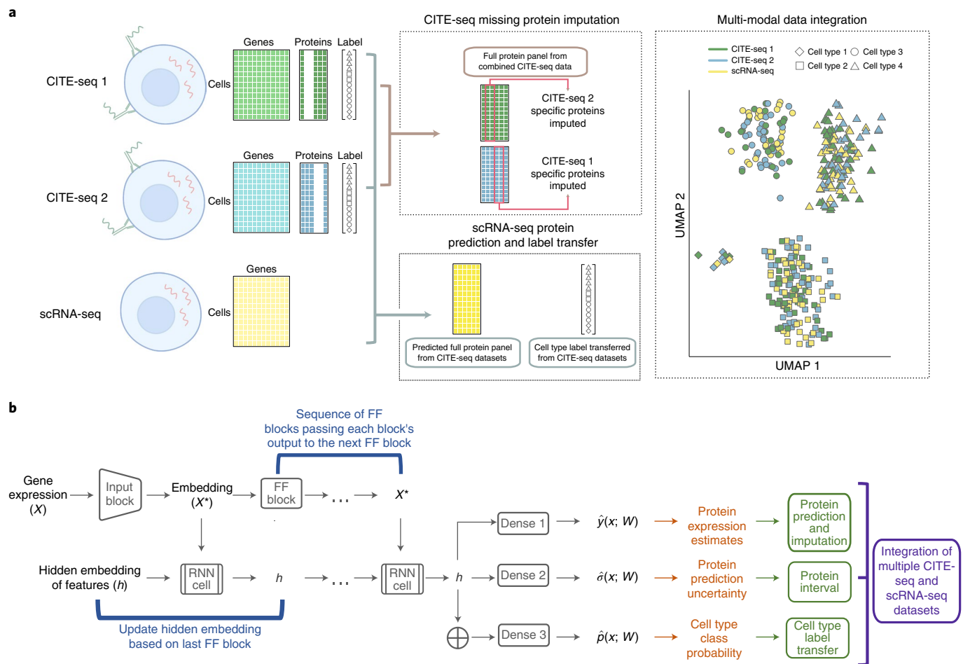
Fig. 1 | Overview of sciPENN. a , sciPENN is a flexible method that supports completion of multiple CITE-seq references (by imputing missing proteins for each reference) as well as protein expression prediction in an scRNA-seq test set, all in one framework. Simultaneously, sciPENN can transfer cell type labels from a training set to a test set, and can also integrate cells from the multiple
