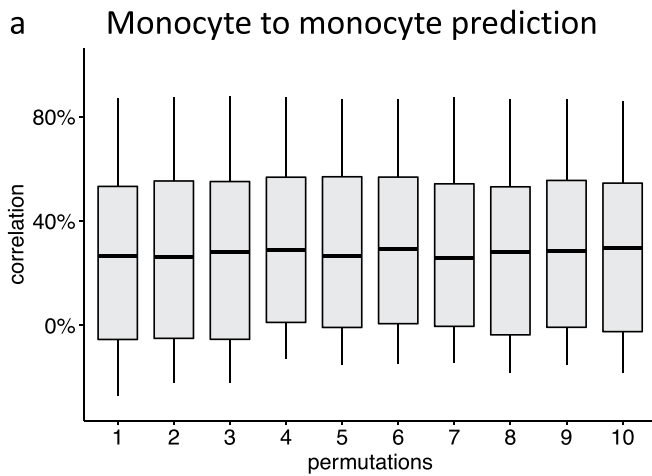
Extended Data Fig. 1 | Evaluation of the robustness of sciPENN by randomly splitting training and testing data. a , Boxplot for correlations between predicted and observed protein expression based on a random split of the Monocyte data into training and testing. The lower and upper hinges correspond to the first and third quartiles, and the centre refers to the median value. The upper (lower) whiskers extend from the hinge to the largest (smallest) value no further (at most) than 1.5 \times interquartile range from the hinge. Displayed are results for 10 random splits. The number of cells in the analysis is 37,122.
