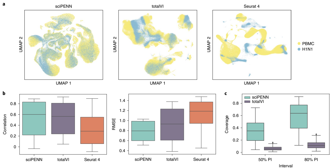
Fig. 5 | Protein expression prediction in the H1N1 dataset using the Seurat 4 PBMC dataset as reference. a , UMAP embeddings visualizing the integrated hidden representation of the data, for each method. Each cell is coloured according to the dataset from which it was sequenced. b , Box plots showing the correlation (left) and the RMSE (right) between each H1N1 protein's predicted and true values for each method. c , Box plots showing the empirical test coverage
