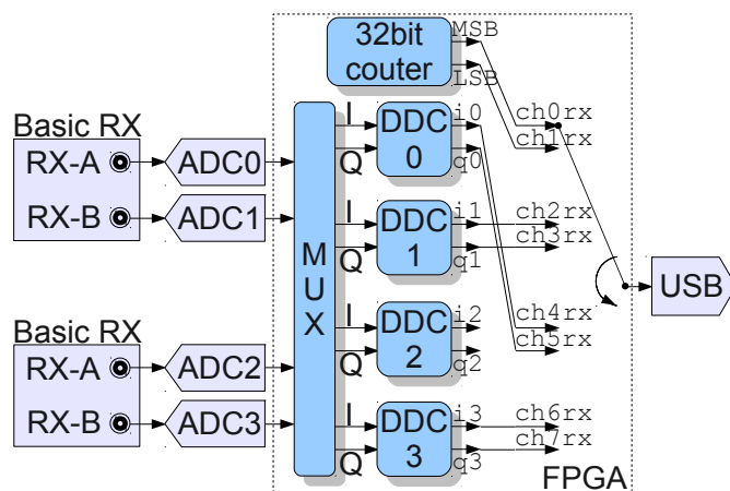
Fig. 4. Configuration of a single USRP in multiUSRP mode.
