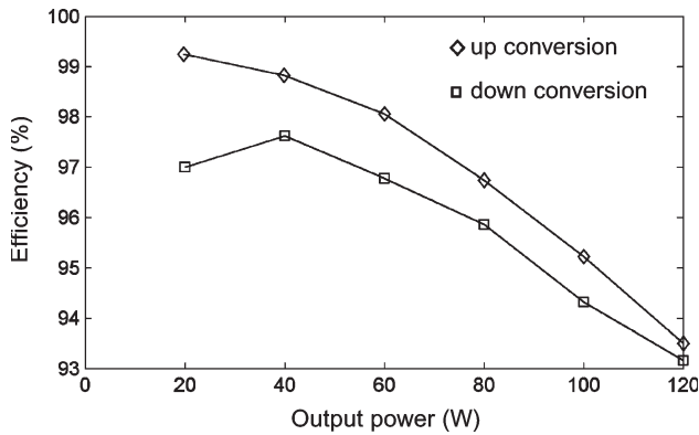
Fig. 13. Efficiency of the MMCCC at different power outputs.
