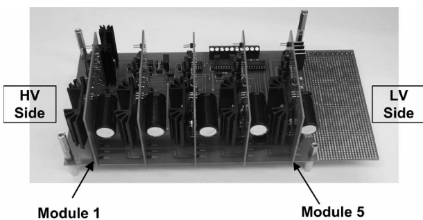
Fig. 14. 500-W six-level prototype.
