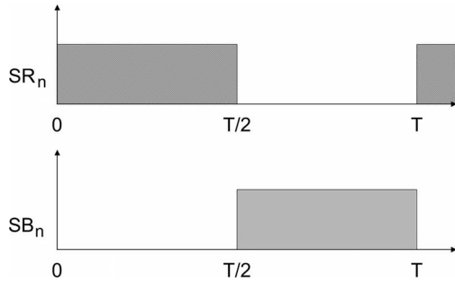
Fig. 6. Gating signal of the switches in the new circuit, i.e., there are only two switching states present in the circuit.
