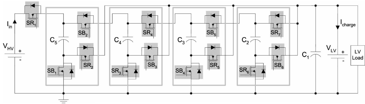
Fig. 3. Five-level MMCCC with four modular blocks.
