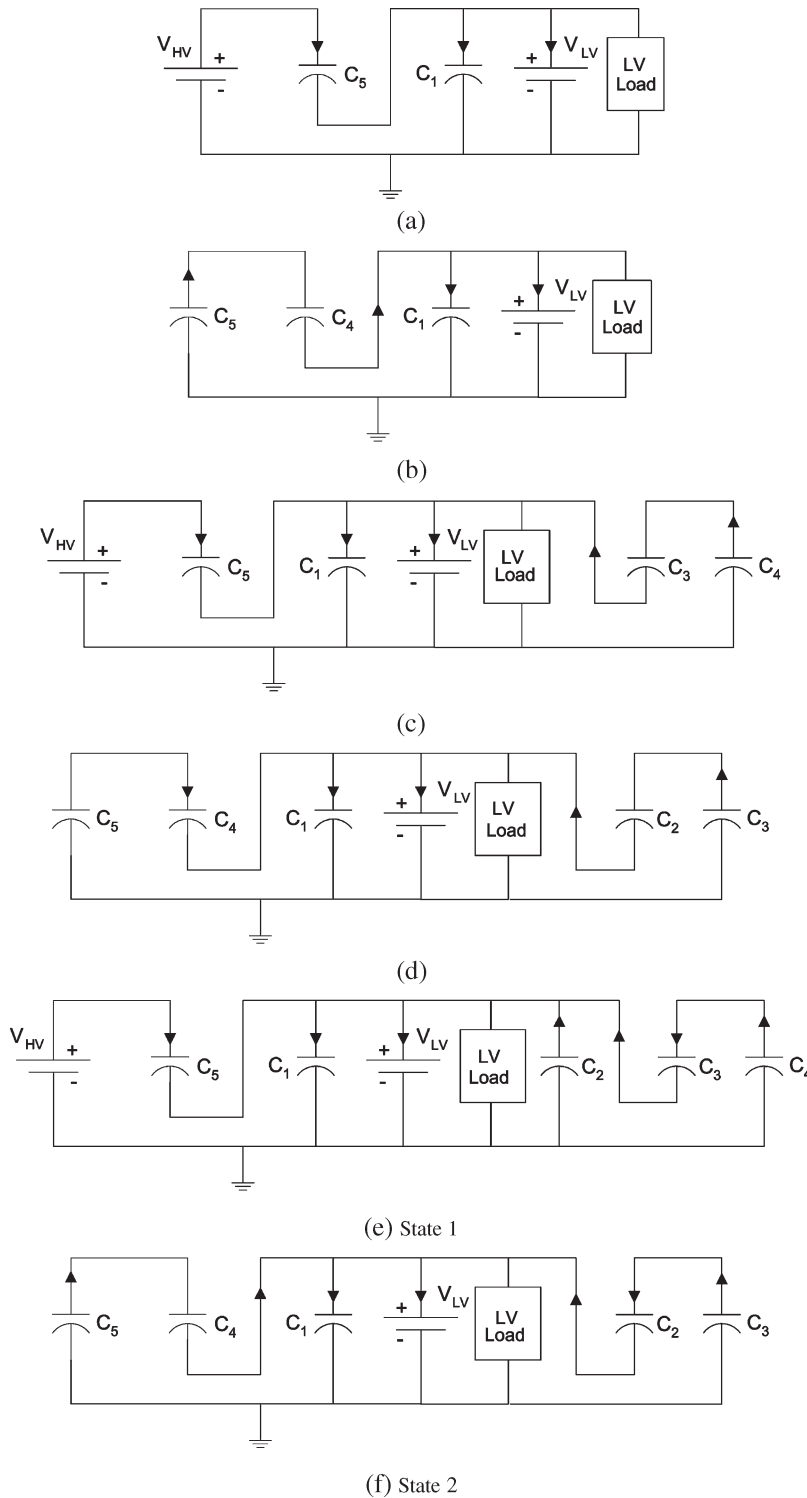
Fig. 5. Simplified diagram of the new converter using the switching scheme of the conventional converter.
