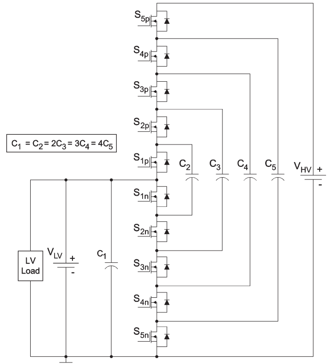
Fig. 1. Schematic of a five-level FCMDC.
