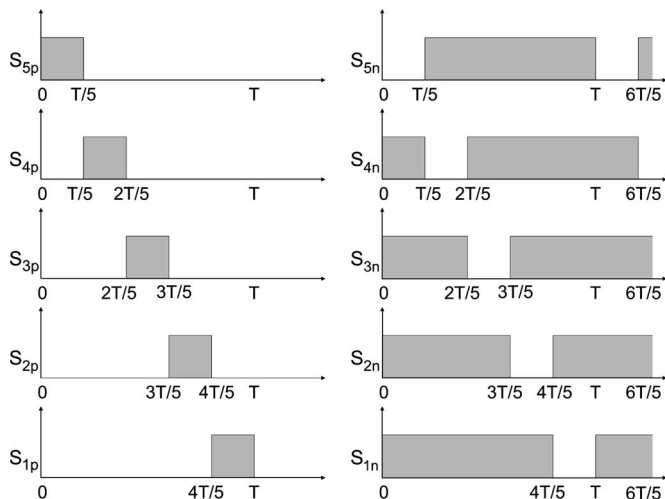
Fig. 2. Switching scheme of the FCMDC circuit.
