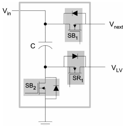
Fig. 4. Modular block of the MMCCC.
