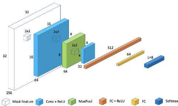
Figure 2. Language Prediction Network . In this figure L = N_{lang} = 8 , denoting the eight scripts (Arabic, Bengali, Chinese, Hindi, Japanese, Korean, Latin and Symbol) supported by our default model in this paper.
