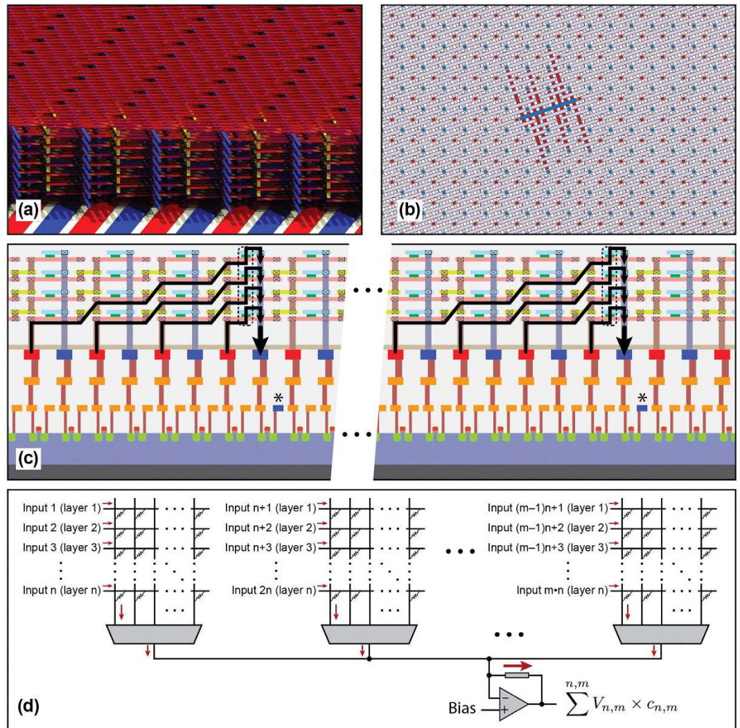
Figure 1. Conceptual representation of a 3D CMOL multiply-add engine. (a) Conceptual view of a 3D multi-layer crossbar integrated on CMOS substrate. The red and blue thinner wires represent the bottom and top electrodes of the crossbar respectively, the thicker red and blue wires illustrate the CMOS interconnections. (b) Top-view of one layer of a CMOL crossbar: the red and blue dots represent the contact vias for the bottom (BE) and top electrodes (TE) respectively. The highlighted electrodes (one TE and eight BE) demonstrate the CMOL connectivity. (c) Cross-sectional view of (b) showing multiply-add operation at the ‘blue’ pin of the eight input signals fed through the eight ‘red’ pins. (d) Multiply-add operation in a (m \times m \times n) 3D crossbar where n is the number of layers.
