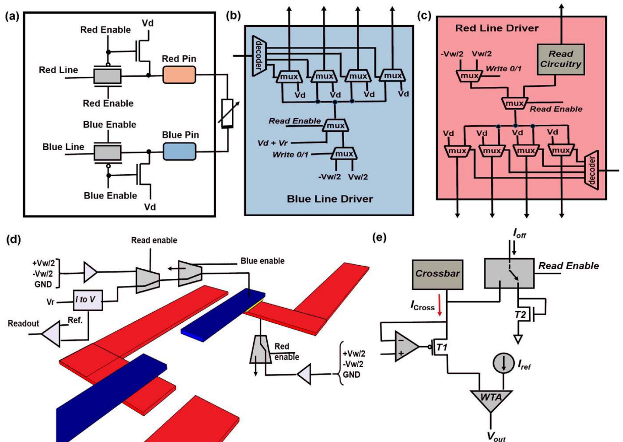
Figure 3. CMOS circuitry. (a) Circuit of a CMOS cell. (b,c) Blue and Red line driver for supplying the appropriate biases to the Blue and Red pins respectively. (d) Cartoon of the write/read operation for the memristive crossbars. (e) Schematic of the sensing circuit.
