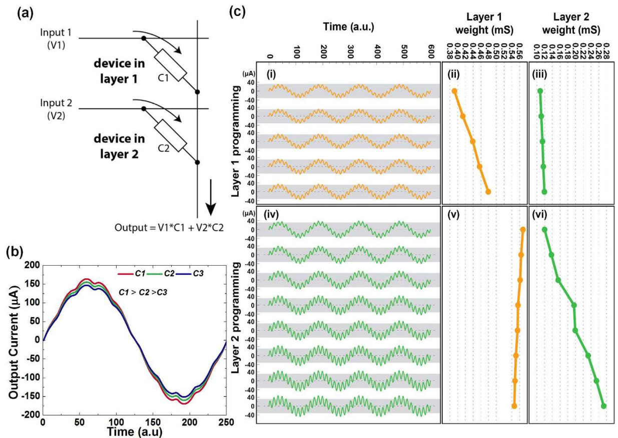
Figure 5. Dot-product operation in the integrated 3D memristive crossbars. (a) Schematic of the set-up for the dot-product operation utilizing two devices in two different layers of the 3D crossbar, (b) An example of the dot product operation with two sinusoidal inputs applied to two devices in a 3D crossbar and the device in layer 1 being programmed to decreasing conductance values, (c) (i) evolution of the output waveform with the weight of the device in layer 1 changing (ii) and the weight for the device on the 2nd layer being kept constant (iii); (iv) evolution of the output waveform when weight of the device in layer 1 is kept constant (v) while layer 2 device changes its state (weight) (vi).
