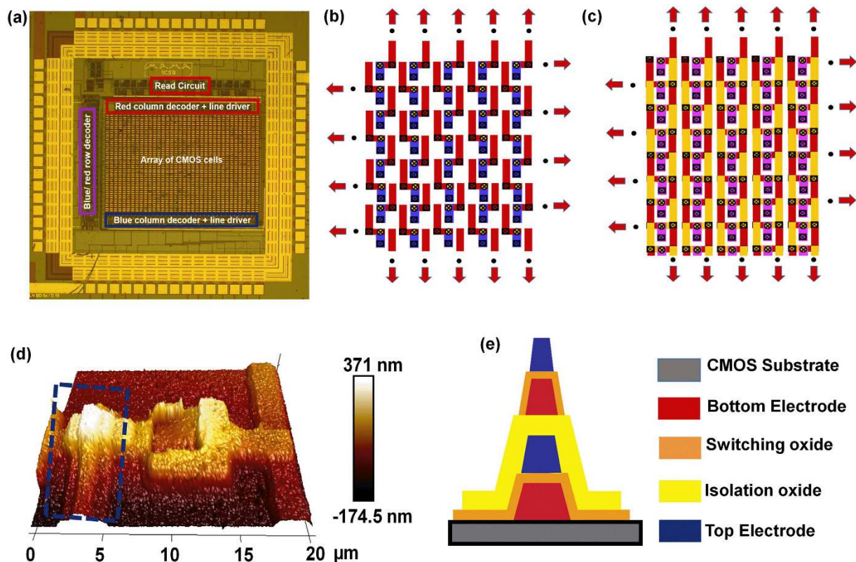
Figure 2. Fabrication of a 3D CMOL crossbar. (a) Optical image of the foundry-processed CMOS chip showing the on-chip decoder, 'Read' and 'Write' circuitry as well as the 24 \times 36 array of CMOS cells. Each 'CMOS cell' houses a pair of pins ('Red' and 'Blue'), (b) structure of the first layer of the 3D crossbar, (c) the final structure of the 3D crossbar with 2 layers (d) AFM image of a section of the 3D crossbar: the highlighted section shows two stacked device layers, (e) Cross-section of the region highlighted in (d).
