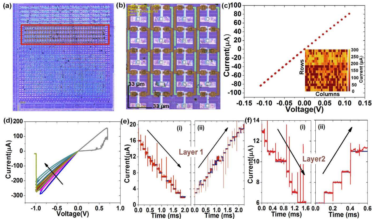
Figure 4. Electrical characteristics. (a) An optical image of the CMOS chip with vertically integrated memristive crossbars: the region highlighted in the red box has the 3D CMOS crossbar structures, (b) A high-resolution optical image of a section of the integrated 3D crossbars. (c) A typical I - V plot measured on a test structure to test the contact resistance between the memristive layer and the underlying CMOS. Inset shows a map of the current measured at all the 24 \times 36 array of 'red pins' showing contact between the integrated devices and the CMOS cells. Current is measured at 0.2 V for each measurement. (d) An I - V plot showing typical DC switching characteristics of the integrated memristive devices: the device is initially turned on and is gradually reset demonstrating analog switching behavior, (e) pulsed switching characteristic of a device in layer 1 showing gradual reset and set operation: the device is tuned to each desired state using a tuning algorithm (discussed in the supporting info.). The arrow indicates the direction of programming in each case, (f) pulsed switching characteristic of a device in layer 2 showing gradual reset and set operation: the device is tuned to each desired state using the tuning algorithm.
