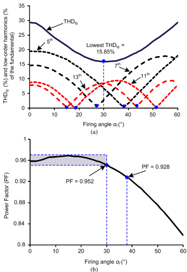
Fig. 8. Simulation results of the multi-rectifier system with different firing angles for the SCR unit: (a) total harmonic distortion and the low-order harmonic distribution of the input current i_g and (b) power factor.
