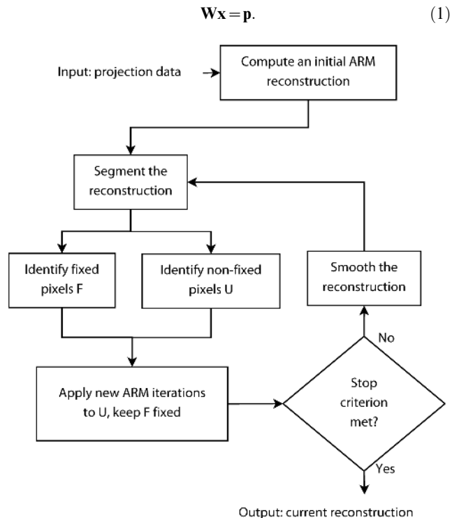
Figure 1. Flow chart of DART [1]. doi:10.1371/journal.pone.0106090.g001
