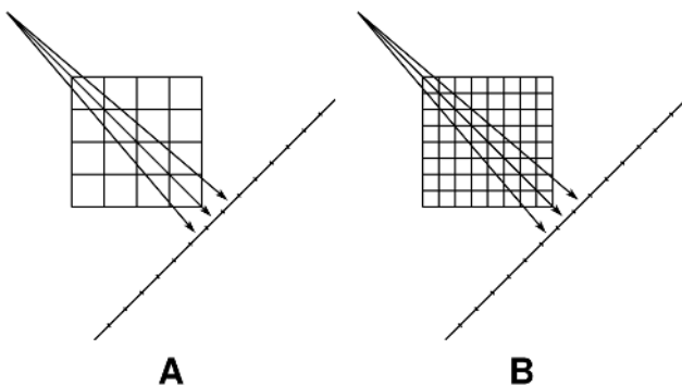
Figure 4. Projection geometry and reconstruction grids used by MDART 2. The coarse reconstruction grid (A) and the target reconstruction grid (B). doi:10.1371/journal.pone.0106090.g004
