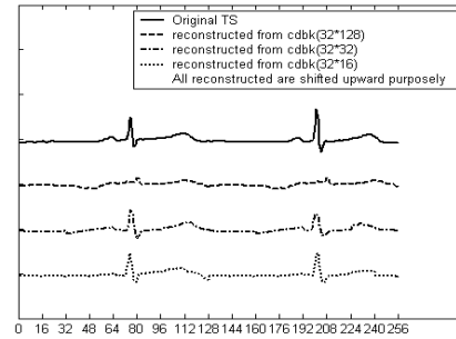
Figure 4. Reconstruction of time series using different resolutions
