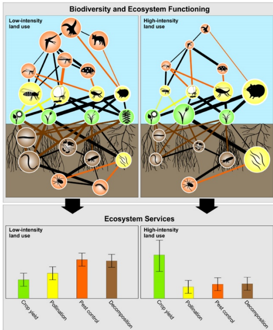
Figure 3 Multitrophic communities drive ecosystem multifunctionality. This scheme depicts relationships between the diversity of species in aboveground-belowground networks and the management of multiple ecosystem services across adjacent agricultural ecosystems. Management decisions, such as intensifying agricultural practices (right part of the figure), that focus on locally maximizing one ecosystem service, such as crop yield, can limit the other ecosystem services provided in complex food webs in a given area (e.g., pest control is reduced, indicated by higher biomass of aphid and vole). Note that the stability of delivering the focal service decreases in this example (larger error bar in crop yield) at high land-use intensity (Isbell et al., 2017b). Socio-political context related to human population density and stakeholder interests can influence feedbacks between ecosystem services and the management of complex ecosystems. Importantly, ecosystem services are not solely provided by single nodes in the food web and at a single location, but by the interaction among multiple nodes (colors of example links between nodes in upper part, correspond to ecosystem service bar colors in lower part) across adjacent ecosystems. Redrawn after Hines et al. (2015b).
