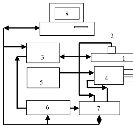
Figure 1. Block diagram of MAPL. 1. Laser head, 2. Si detector, 3. Laser power supply and control, 4. optical receiver package, 5. high voltage supply for PMT detector, 6. Digital delay pulse generator, 7. Digitizer and 8. computer.
