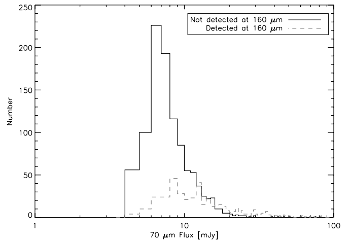
Figure 18. 70 \mu\text{m} flux distribution of the 463 sources detected at 160 \mu\text{m} (gray dashed) and the 1042 not detected at 160 \mu\text{m} (solid black). On average, those detected at 160 \mu\text{m} have higher 70 \mu\text{m} fluxes.
