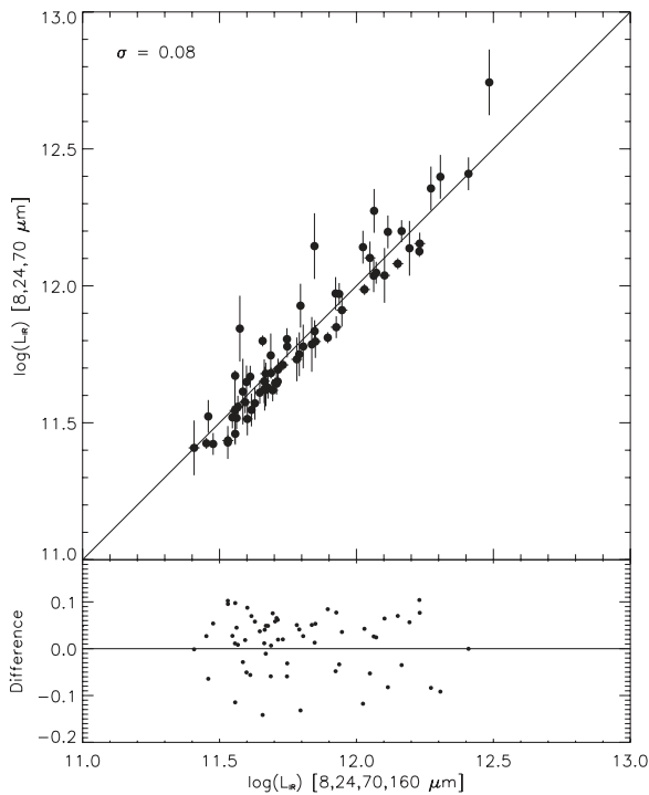
Figure 16. Comparison of the total infrared luminosity obtained with and without the 160 \mu\text{m} data point for a sample of 67 local (U)LIRGs from the GOALS survey. The low dispersion obtained between these two measures indicates that the template fitting method is reliable and that the rest-frame 70 \mu\text{m} data point is long enough to obtain a reliable measure of L_{\text{IR}} at low redshift ( z < 0.1 ).
