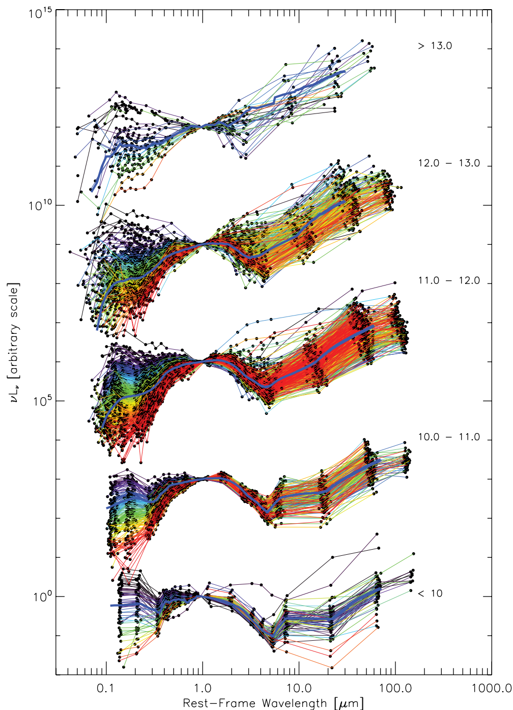
Figure 21. SEDs of all 1503 70 \mu\text{m} sources binned by luminosity and normalized at 1 \mu\text{m} . The SEDs are color coded such that the ones with the bluest slope in the UV–optical are purple/blue and the reddest are red and the spectrum in between shows the range of SED colors. The median SED for each bin is overplotted in blue. Note the large variety in SED shapes, particularly in the UV, and the trends with L_{\text{IR}} . At the highest luminosities, there is an obvious trend toward power-law SEDs all the way from the optical through the FIR.
