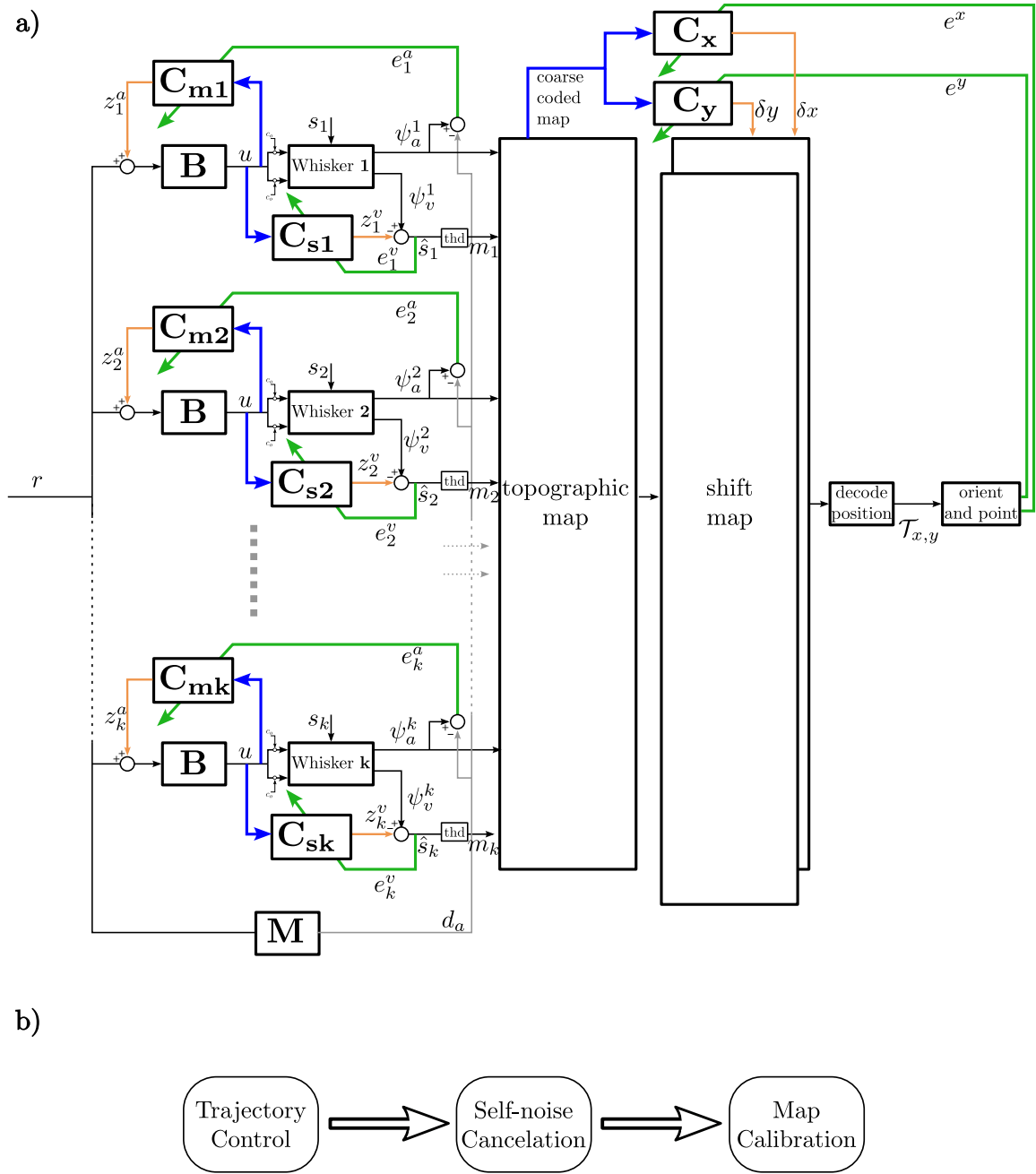
Figure 5. Schematic of the overall control architecture. a) The architecture for implementing the cerebellar algorithm simultaneously in three distinct areas is shown for k whiskers. For trajectory control and sensory noise cancellation, 2 \times k separate cerebellar microzones are used. The microzones for trajectory control and sensory noise cancellation corresponding to the k^{th} whisker are denoted C_{mk} , and C_{sk} respectively. The outputs write into a single topographic map. Two microzones ( C_x , C_y ) are used to shift the map in the x, y directions to correct for errors in orienting to novel targets. b) Pipeline of tasks that the cerebellar algorithm is applied to.
