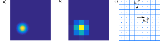
Figure 4. Example of coarse coding for map calibration. a) Example of 2D topographic map providing a probabilistic representation of the location of a detected target. b) Coarse-coded, normalised version of the topographic map, here an 8x8 grid is used to represent the coarse coded image. c) Example of estimated x, y weights for the i^{th} parallel fibre.
