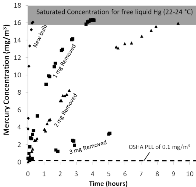
Figure 2. Equilibrium mercury vapor concentrations above CFL debris, and rate of approach to the equilibrium values in a 0.5 L flask. Although most Hg is associated with the phosphor, glass, or endcaps, its equilibrium vapor pressure is similar to that of free liquid Hg and over 150 times the OSHA-PEL. Partial removal of Hg (1, 2, and 3mg) by heating and gas purging reduces the release rates, but does not affect the equilibrium vapor concentrations. After 3 mg removal, the equilibrium Hg concentration returns to >15,000, but over 30 hours (data not shown). This equilibrium data is relevant to Hg-vapor concentrations expected in small confined spaces.
