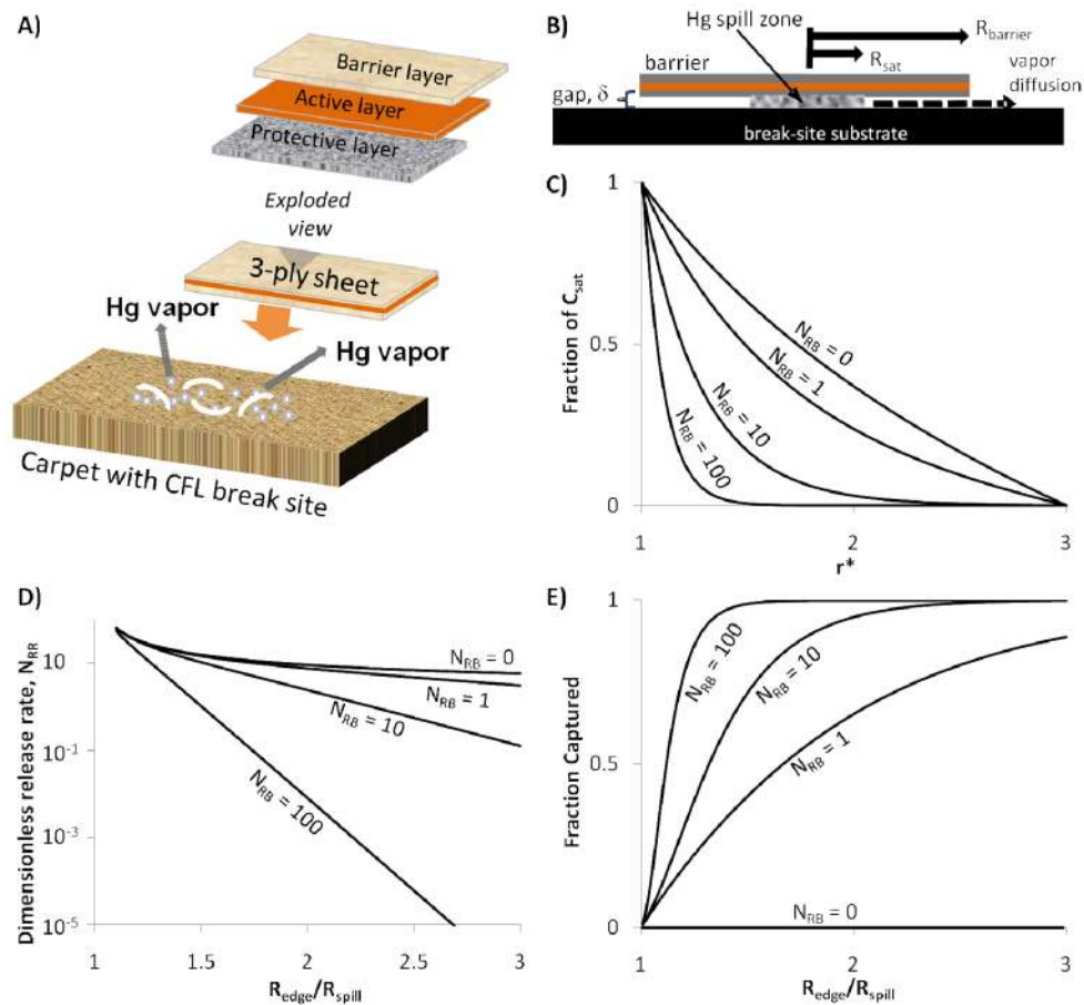
Figure 3. Formulation and prediction of a coupled reaction and transport model of the reactive barrier technology applied to fluorescent lamp break sites. A) Exploded view of reactive barrier concept, B) Model formulation, C) Example Hg concentration profiles under a barrier three times the size of the spill, D) Release rates as a function of the dimensionless barrier number, N_{RB} , and ratio of reactive barrier size R_{edge} to spill size R_{spill} , E) Predictions of the fraction captioned of the mercury leaving the saturated zone.
