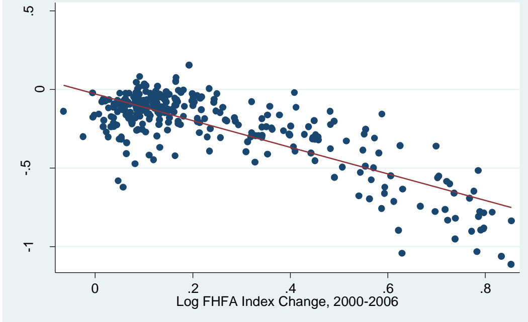
Figure 2: Mean Reversion in MSA Housing Prices 2000-2006 and 2006-2012
