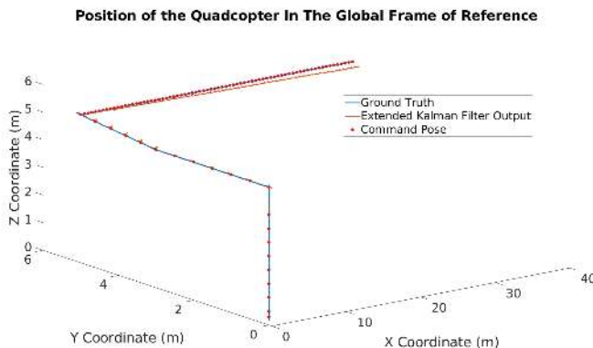
Figure 6. EKF pose estimation
