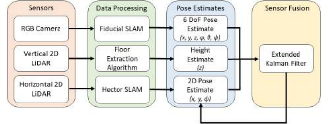
Figure 1. Software Architecture for the Proposed Navigational System.
