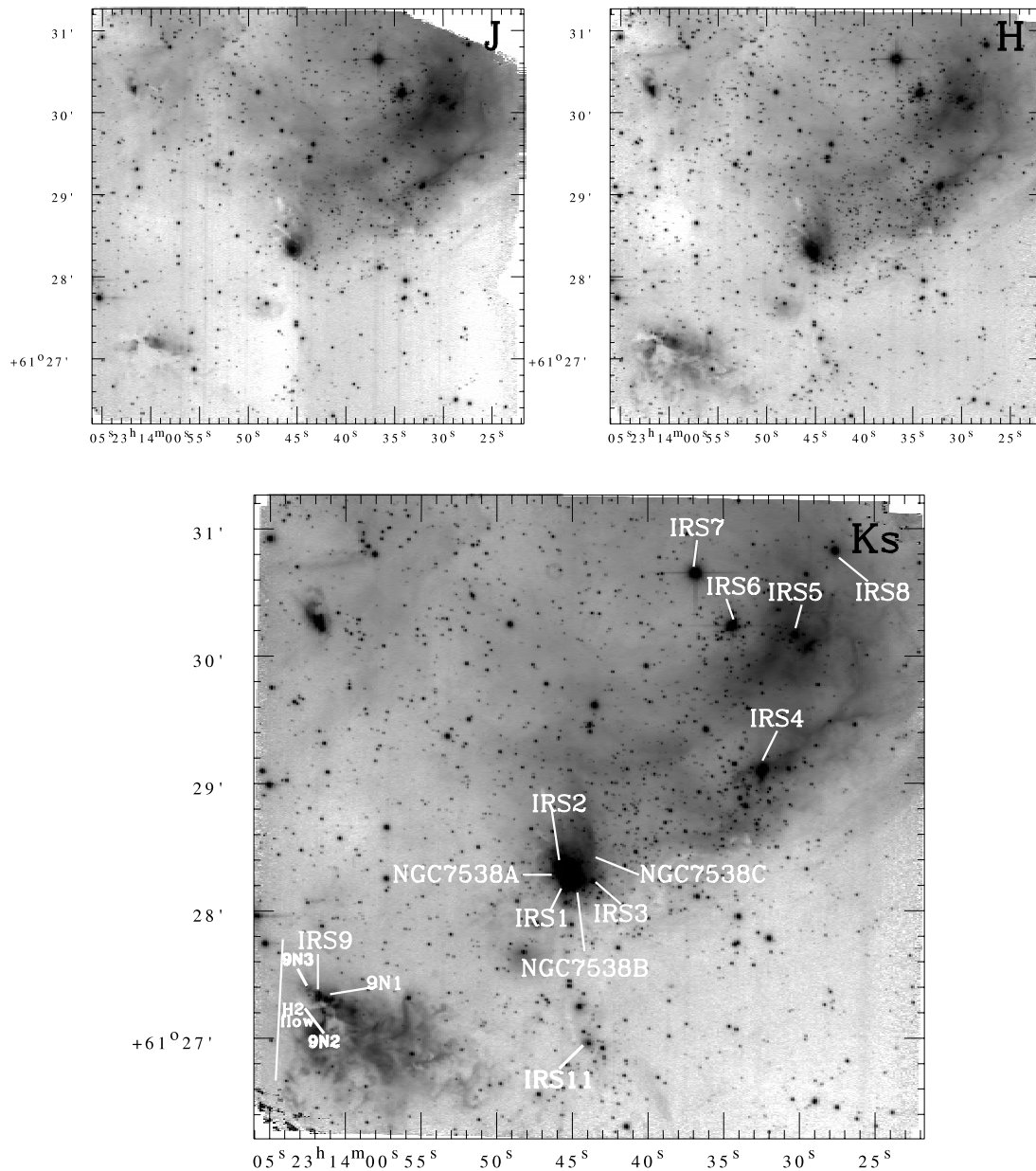
FIG. 1.— J -, H -, and K s -band images of the NGC 7538 star-forming region displayed in a logarithmic intensity scale. The FOV is \sim 4'.9 \times 4'.9 . The locations of the individual IR sources are marked in the K s -band image. The direction of the NGC 7538 IRS 9 “H 2 flow” reported by Davis et al. (1998) is also indicated in the K s -band image. North is up, and east is to the left. The abscissa and the ordinate are in the J2000.0 epoch.
