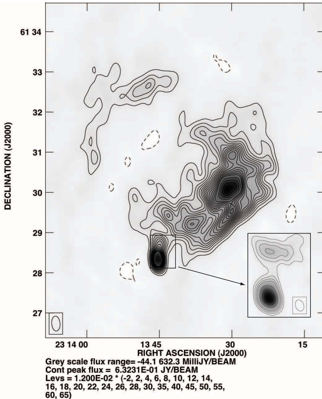
FIG. 2.—GMRT low-resolution map of the whole NGC 7538 region at 1280 MHz. The resolution is 22''.5 \times 12''.4 along P.A. = 4^\circ.6 , and the rms noise in the map is \sim 4 mJy beam ^{-1} . The abscissa and the ordinate are in the J2000.0 epoch. The inset is a GMRT high-resolution map of the central radio peak. The image has a high resolution of 6''.6 \times 4''.7 along P.A. = 21^\circ.4 , an rms of \sim 1.3 mJy beam ^{-1} , and a total flux density of 978.7 mJy. The lower part of the map is the same area as the JHK s image (see Fig. 4).
