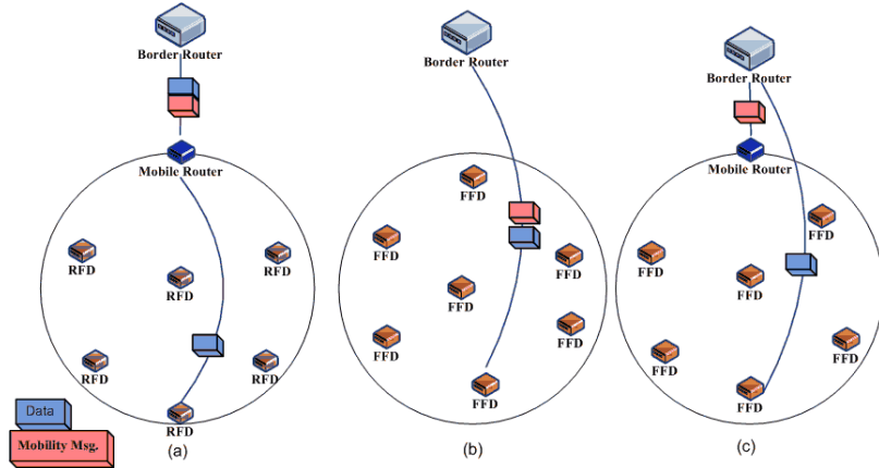
Fig. 7. The Messages Scheduling of Three Models. (a) RFD Devices with MR, (b) FFD Devices without MR, (c) FFD Devices with MR
